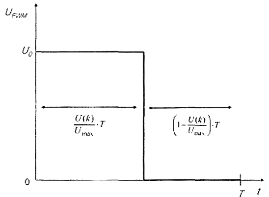
Fig. 3 Duty ratio of PWM algorithm
