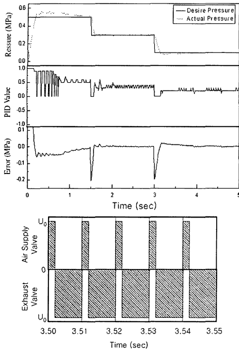
Fig. 11 Experimental results of decreasing step response by conventional PWM
