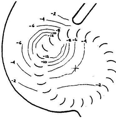
(a) Static pressure by Mazur et al. 3
