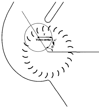
(a) Definition of local coordinates
