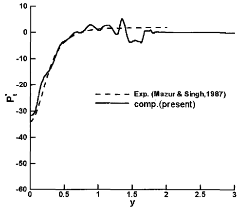
(c) Total pressure variation
