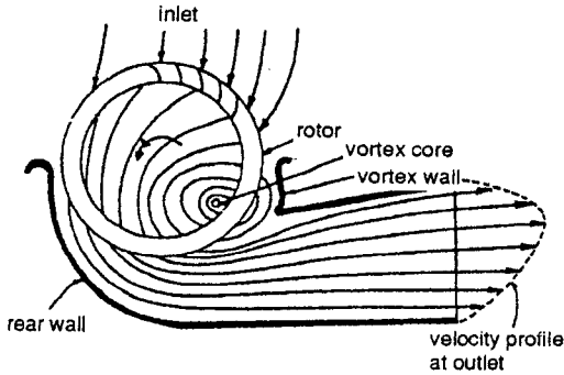
Fig. 1 Diagram of the flow through a cross-flow fan
