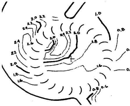
(g) Total velocity by Mazur et al. 3
