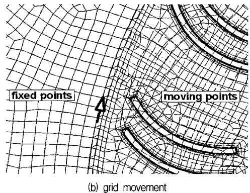
Fig. 2 Moving grid for the cross flow fan
