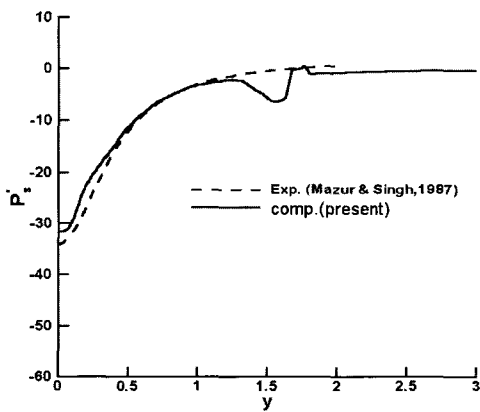
(b) Static pressure variation
