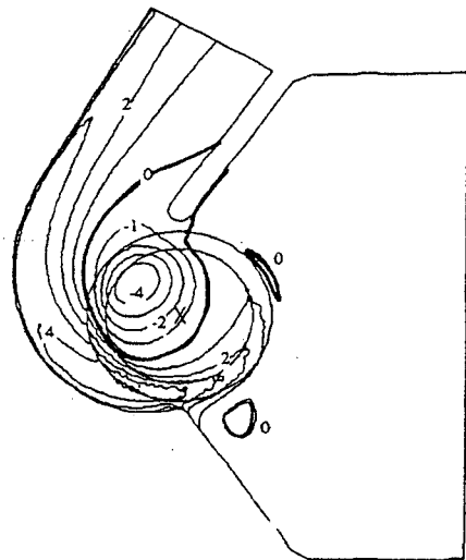
(e) Total pressure by Combes et al. 10
