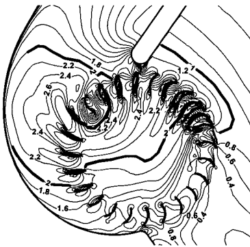
(h) Present total velocity
