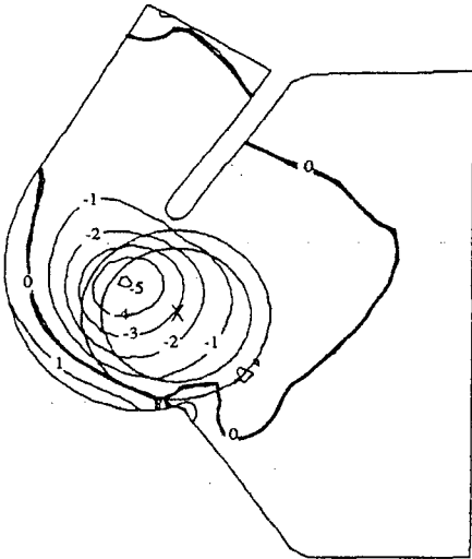
(b) Static pressure by Combes et al. 10
