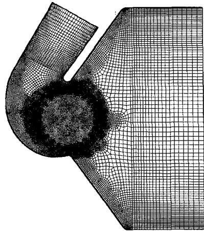
Fig. 3 Computational grid
