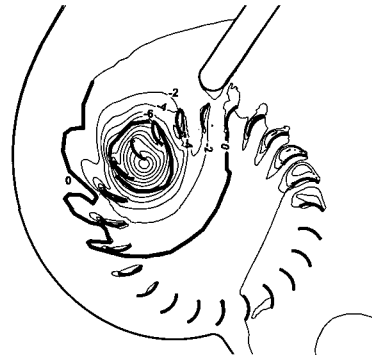
(f) Present total pressure
