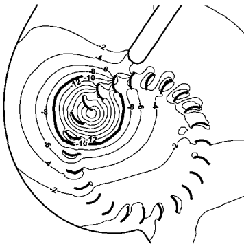
(c) Present static pressure
