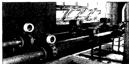
Fig. 3 Reference flowmeters
