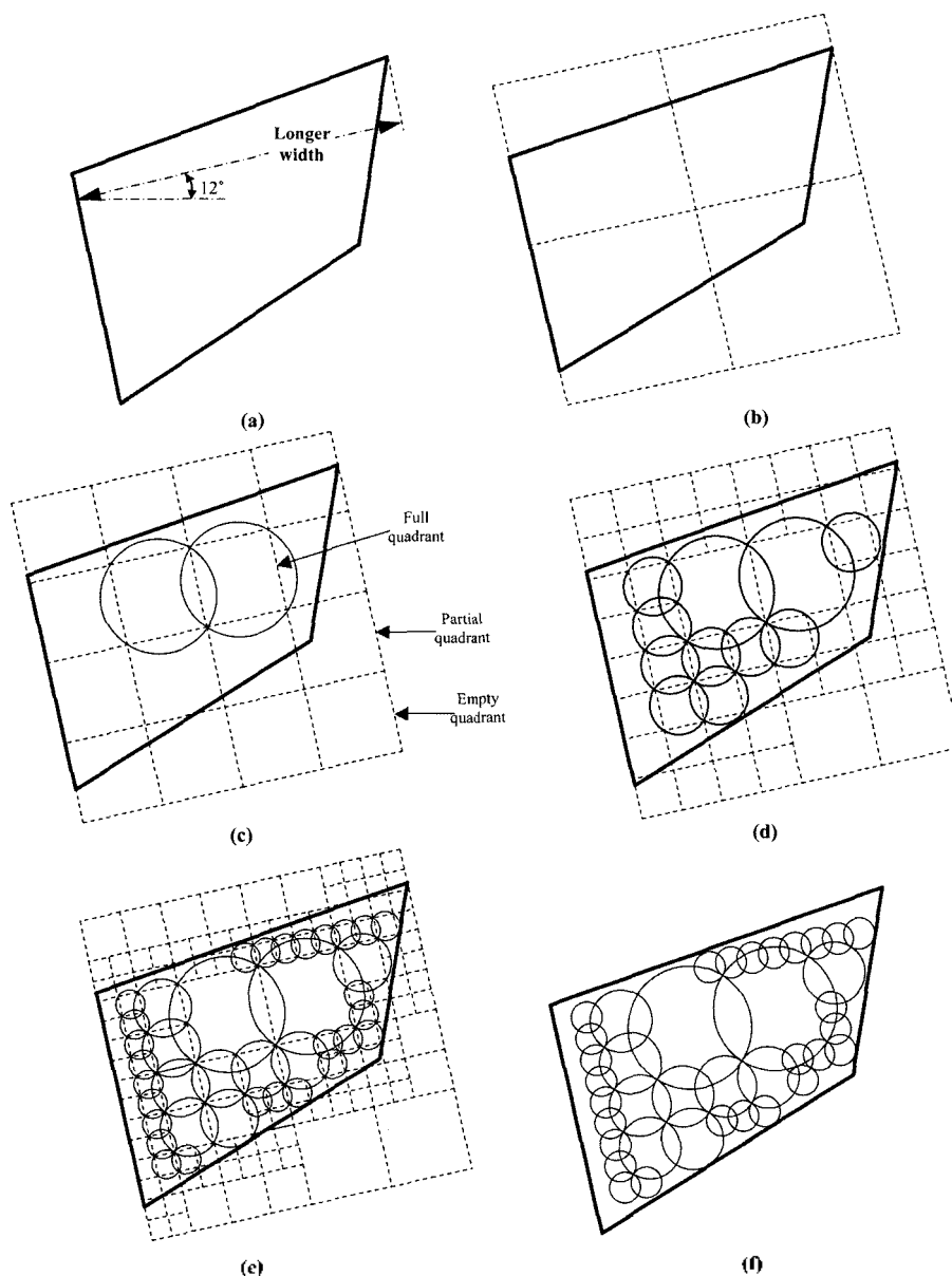
Fig. 7. Proposed method to fill the plunged area (Continued). (e) 4 th step of splitting enclosed square, (f) Plunge-milling toolpoint path with the desired resolutions. (Three plungers)
