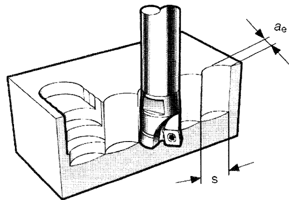
Fig. 1. Plunge-milling cutting process.
