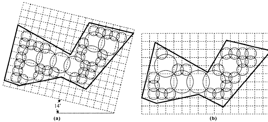
Fig. 9. Comparison of proposed and previous methods. (a) Proposed method (Angle of filling =166, Accessible Volume: 31046.9384), (b) Previous method. (Angle of filling =0.0, Accessible Volume: 29893.6671)
