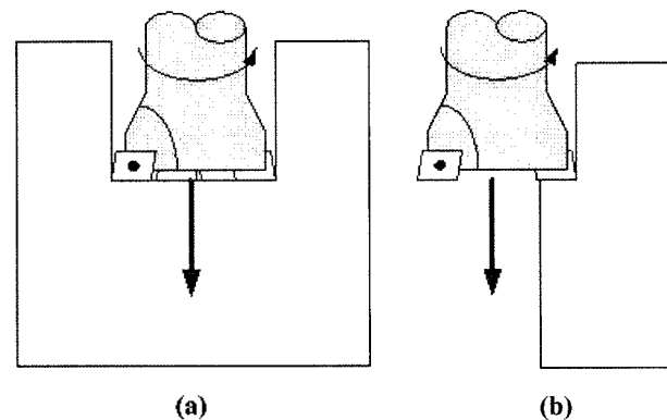
Fig. 2. Plunge-milling cutters. (a) Center plunger, (b) Side plunger.
