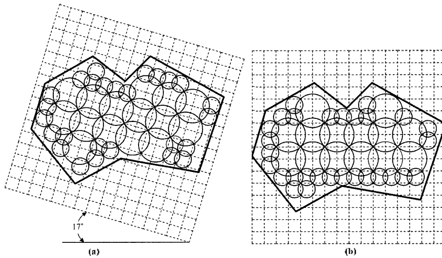
Fig. 8. Comparison of proposed and previous methods. (a) Proposed method (Angle of filling =163, Accessible Volume: 10433.6470), (b) Previous method. (Angle of filling =0.0, Accessible Volume: 10219.0871)
