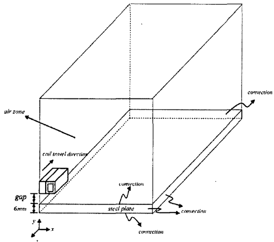
Fig. 4 Schematic half diagram and boundary conditions for FEM
