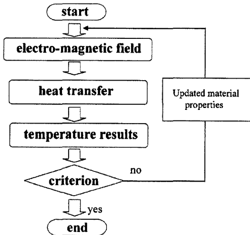
Fig. 2 Simulation procedure flow chart
