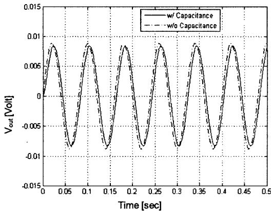
Fig. 6 Simulation of the strain response of the SWCNT/PMMA 10% sensor on a cantilever beam
