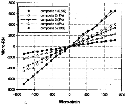
Fig. 2 Strain modeling of SWCNT/PMMA composite sensors with different weight percentages of nanotubes in the PMMA
