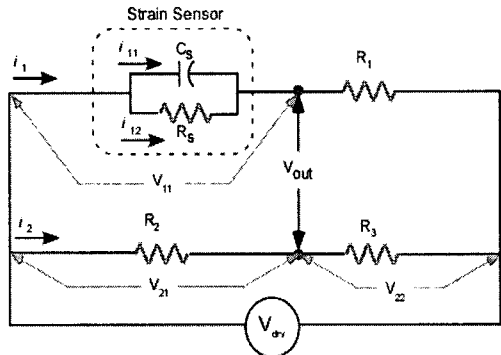
Fig. 5 Sensor output using Wheatstone bridge circuit
