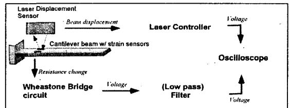
Fig. 7 Test setup of the SWCNT based strain sensor to measure dynamic strain
