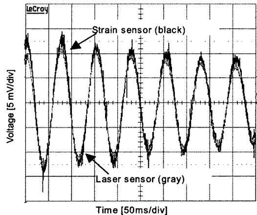
Fig. 8 Dynamic strain response of the SWCNT/PMMA 10% strain sensor in free vibration beam (cutoff frequency 30 Hz, gain : 20 dB)
