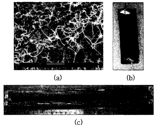
Fig. 1 Fabrication of CNT/PMMA strain sensors (a) SEM images of multi-wall carbon nanotube (MWCNT)/PMMA (20 wt%) sample at 25000x; (b) SWCNT/PMMA sensor (5 wt%, 5 \times 30 \times 0.3 mm, resistivity = 58 cm/S); and (c) fabricated MWCNT/PMMA sensor sprayed on a glass fiber beam (5 wt% MWCNT, 330 \times 5 \times 0.08 mm, R=117.03 k \Omega , C=14.7 pF)
