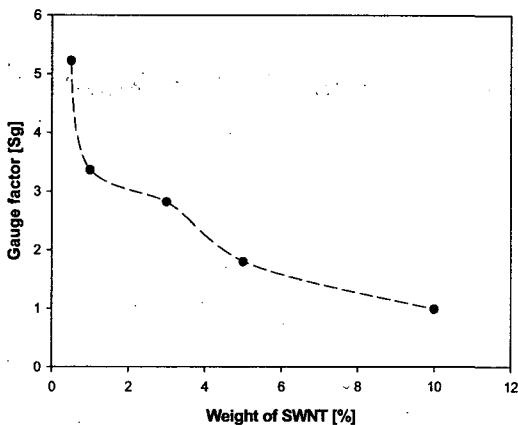
Fig. 3 Gage factor of PMMA /SWCNT strain sensors
