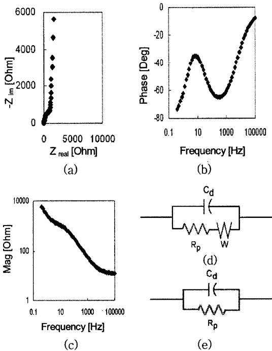
Fig. 4 Dynamic EIS impedance test of 10 % (wt.) SWCNT/PMMA composite sample in 3 % NaCl electrolyte ( R_p = 1.15 \text{ k}\Omega , C_d = 3.5 \mu\text{F} , W = 175.3 \mu\text{S} ) and equivalent electrical models : (a) Nyquist diagram; (b) Bode diagram (phase); (c) Bode diagram (magnitude) (d) Equivalent electrical model of a 10 % (wt.) SWCNT/PMMA composite and (e) simplified electrical model of CNT composite strain sensor
