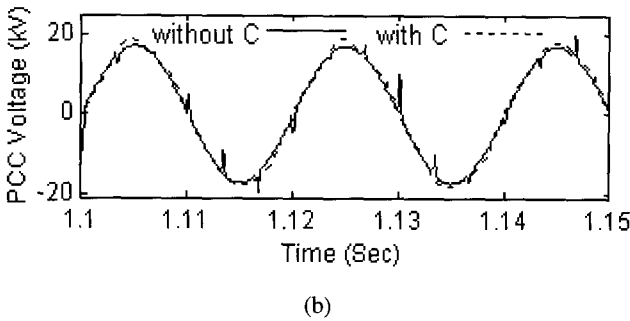
Fig. 7 Passive filters effect (a) Load current (b) Voltage notching
