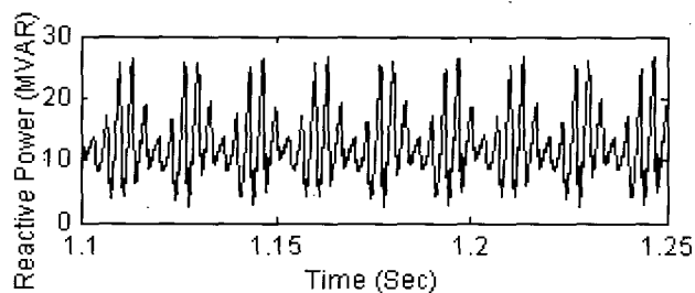
Fig. 14 Load instantaneous reactive power
