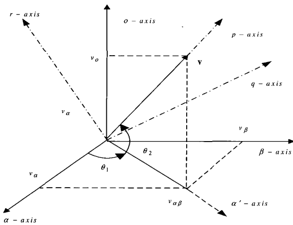
Fig. 2 Relation between \alpha\beta and pqr reference frames
