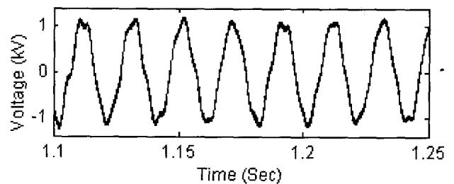
Fig. 10 Series active filter 1 generated voltage, phase-a.
