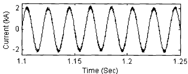
Fig. 12 Series active filter 2 current, phase-a.
