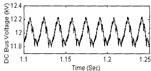
Fig. 16 DC bus capacitor voltage
