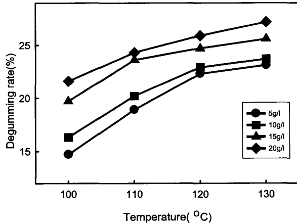
Fig. 5. Effect of degumming temperature on degumming rate at various soap concentration.
