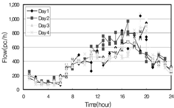
Fig. 3. Flow distribution of on-ramp A
