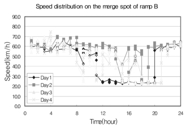
Fig. 8. Speed distribution of on-ramp B
