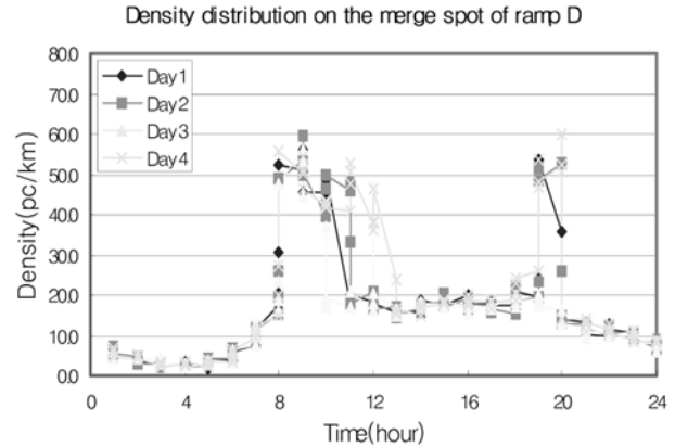
Fig. 14. Density distribution of on-ramp D
