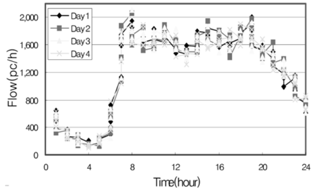
Fig. 5. Flow distribution of on-ramp C
