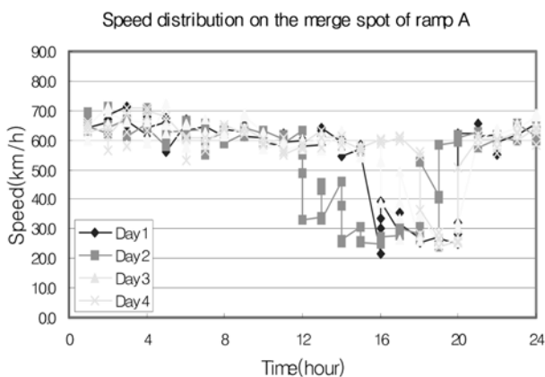
Fig. 7. Speed distribution of on-ramp A
