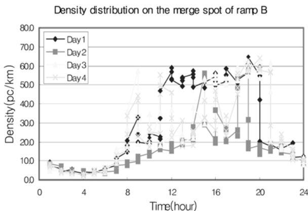
Fig. 12. Density distribution of on-ramp B
