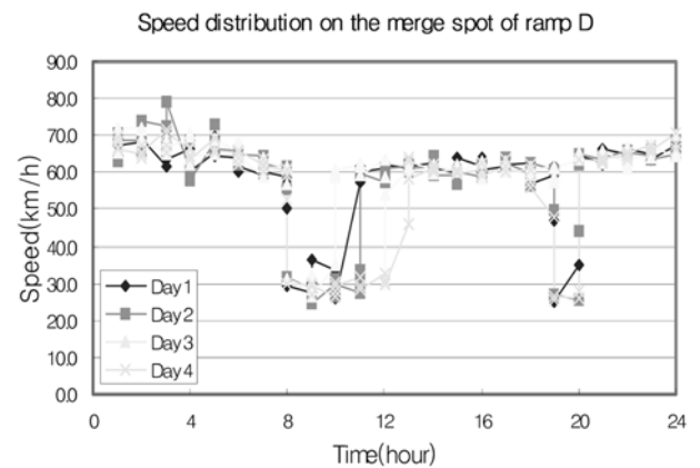
Fig. 10. Speed distribution of on-ramp D
