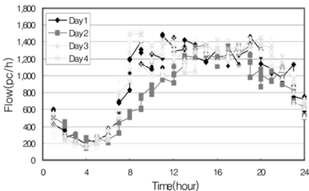
Fig. 4. Flow distribution of on-ramp B
