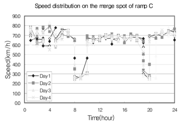
Fig. 9. Speed distribution of on-ramp C
