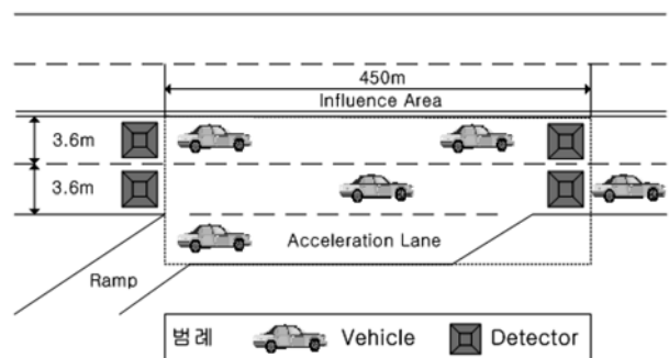
Fig. 1. On-ramp geometry under the study
