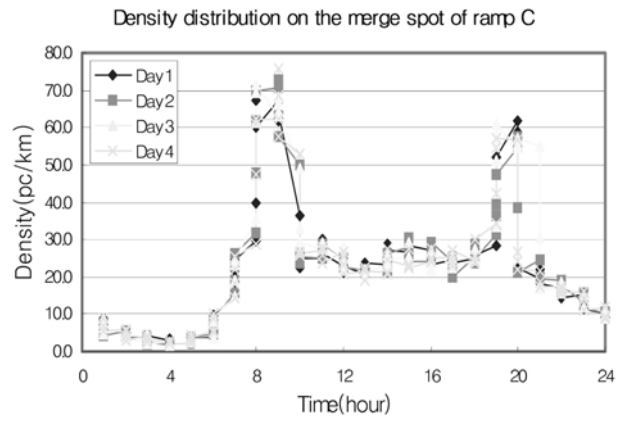
Fig. 13. Density distribution of on-ramp C
