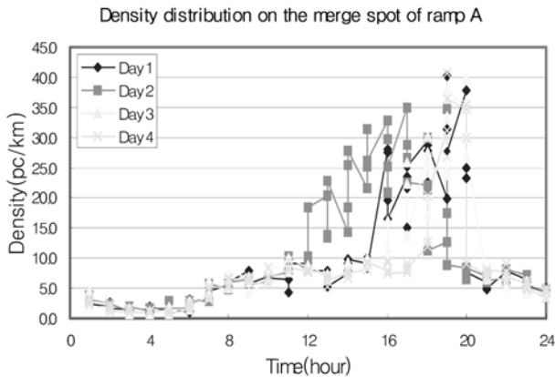
Fig. 11. Density distribution of on-ramp A
