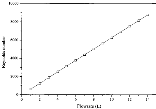
Fig. 9 Reynolds numbers in different flow rate
