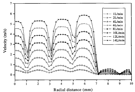
Fig. 7 Velocity distribution of radial direction by volume flow rate change of cooling water
