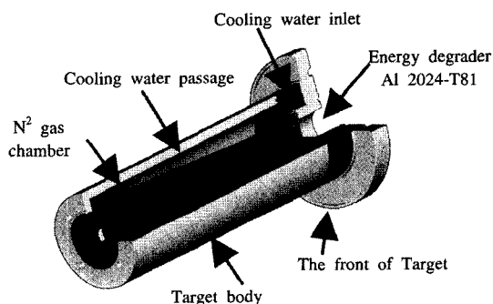
Fig. 1 Overview of gas target
