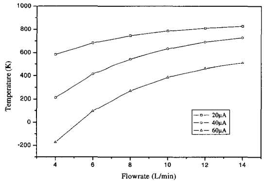
Fig. 20 Temperature requirement of \text{N}_2 gas chamber by current change of proton beam
