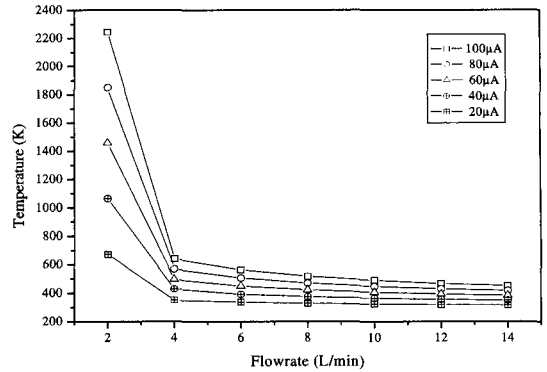
Fig. 14 Maximum temperature of aluminum foil by volume flow rate change of cooling water
