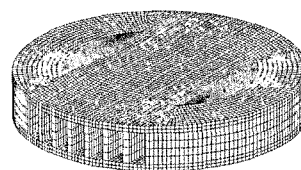
Fig. 4 FEA model of energy degrader
