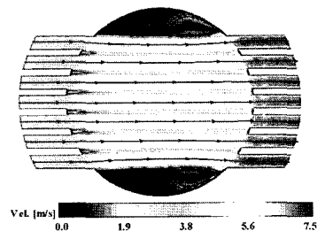
Fig. 8 Flow fields of cooling water in different flow rate (cooling water flow rate : 14 ℓ/min)
