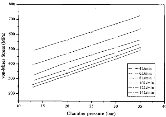
Fig. 18 Maximum stress change of aluminum foil on the gas chamber side by pressure change of \text{N}_2 gas(Proton beam current : 40\mu\text{A} )
