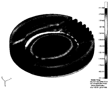
Fig. 16 Example of Von-Mises stress map(proton beam : 40\mu\text{A} , cooling water flow rate : 4\ell/\text{min} , \text{N}_2 gas pressure : 21bar)
