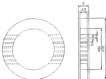
Fig. 2 Dimension of energy degrader
