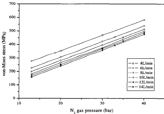
Fig. 17 Maximum stress change of aluminum foil on the gas chamber side by pressure change of \text{N}_2 gas(Proton beam current : 20\mu\text{A} )
