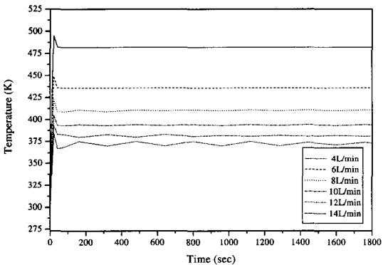
Fig. 13 Maximum temperature distribution in the energy degrader according to time variance(Proton beam current : 60 \mu A)
