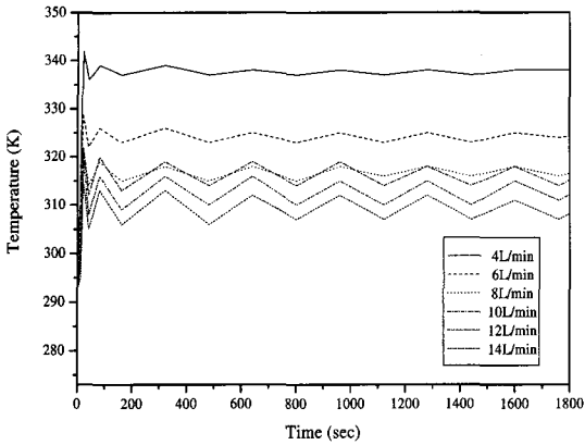
Fig. 12 Maximum temperature distribution in the energy degrader according to time variance(Proton beam current : 20 \mu A)
