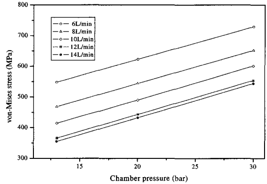
Fig. 19 Maximum stress change of aluminum foil on the gas chamber side by pressure change of \text{N}_2 gas(Proton beam current : 60\mu\text{A} )
