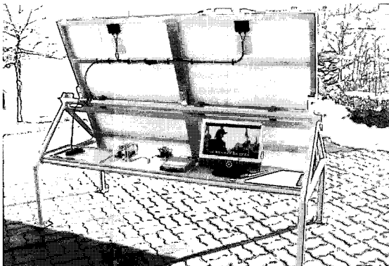
(b) 무접점전원장치 적용 LCD TV및 DVD Player 구동 동작사진 (b) LCD TV and DVD player operating by the use of a contact-less power supply
