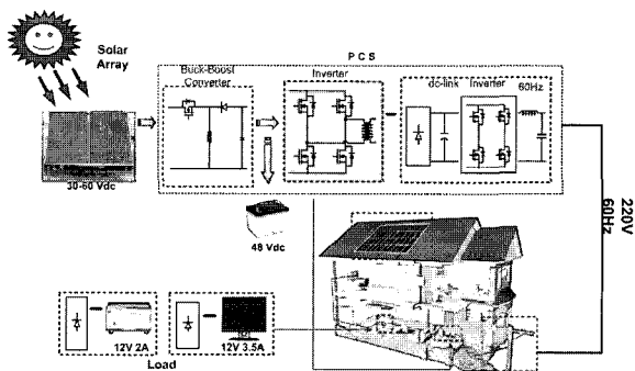
(a) 계통 연계형 태양광 발전 시스템 (a) Utility interactive photovoltaic power generation system for domestic applications
