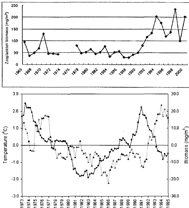
Fig. 3. Zooplankton biomass in the southwestern East/ Japan Sea off Korea ( 35^{\circ}\text{N}\sim 38^{\circ}30'\text{N} , 128^{\circ}30'\sim 133^{\circ}\text{E} ) (Kang and Lee 2002) (A), Anomalies of zooplankton biomass (wet weight, circle) and integrated mean temperatures (0~150m, triangle) along PM line ( 36^{\circ}\text{N} , 136^{\circ}\text{E}\sim 41^{\circ}\text{N} , 132^{\circ}\text{E} ) (B) (Minami et al. 1999).
