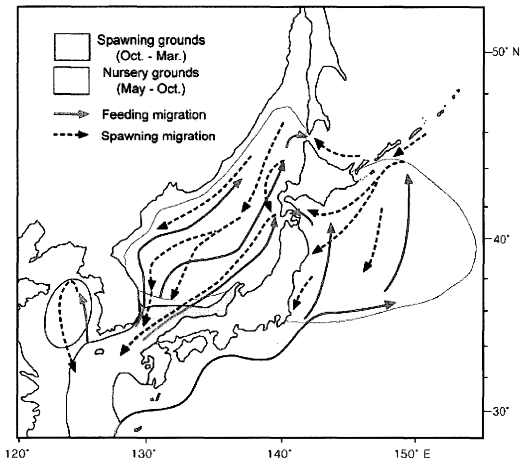
Fig. 12. Hypothetical migration circuits of Todarodes pacificus in the East/Japan Sea and its adjacent waters. Fishing ground ranges from the northern spawning ground to the entire nursery grounds.
