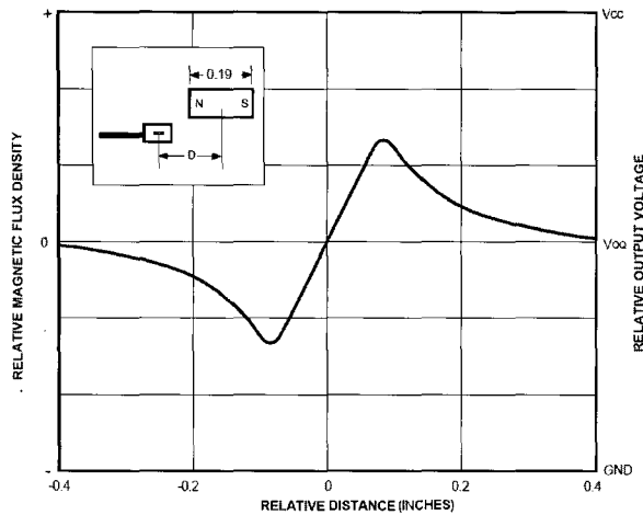
Fig. 2. Hall output voltage in slide-by sensing [6].
