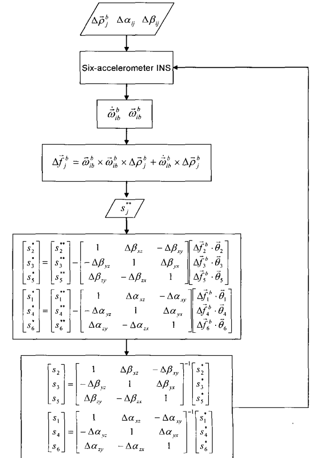
Fig. 3. Six-accelerometer INS compensator.
