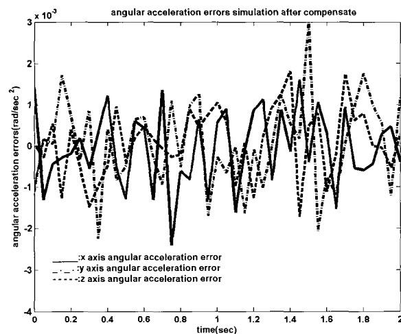
Fig. 10. Angular acceleration errors after compensation.
