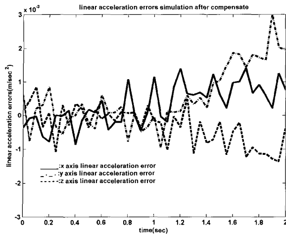
Fig. 9. Linear acceleration errors after compensation.
