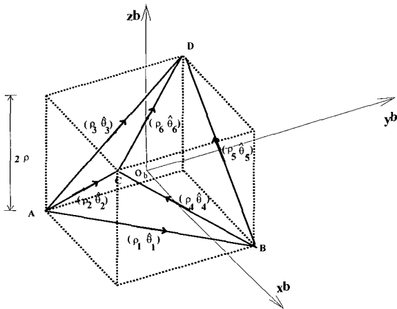
Fig. 2. Six-accelerometer scheme.
