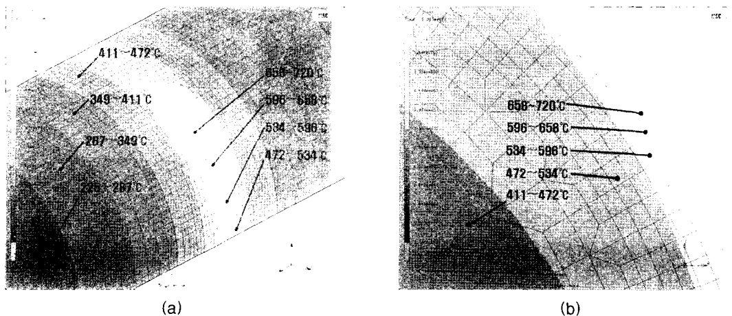
Fig. 8 The resulted temperature distribution on : (a) surface and (b) cross section using MARC
