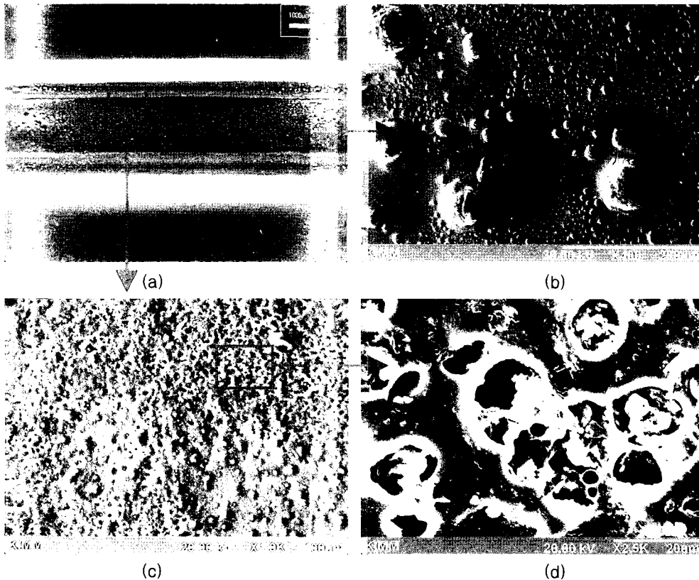
Fig. 4 SEM images of surface at 1700°C under the No.5 condition
