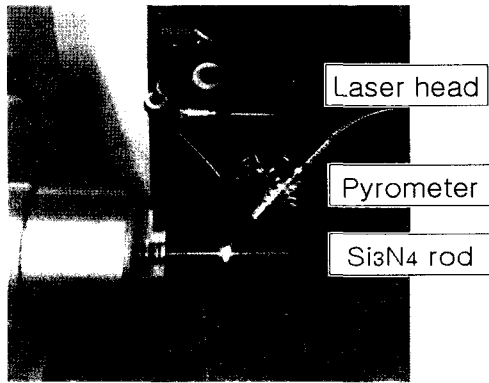
Fig. 1 Experiment system for CO 2 laser irradiation on Si 3 N 4 rod
