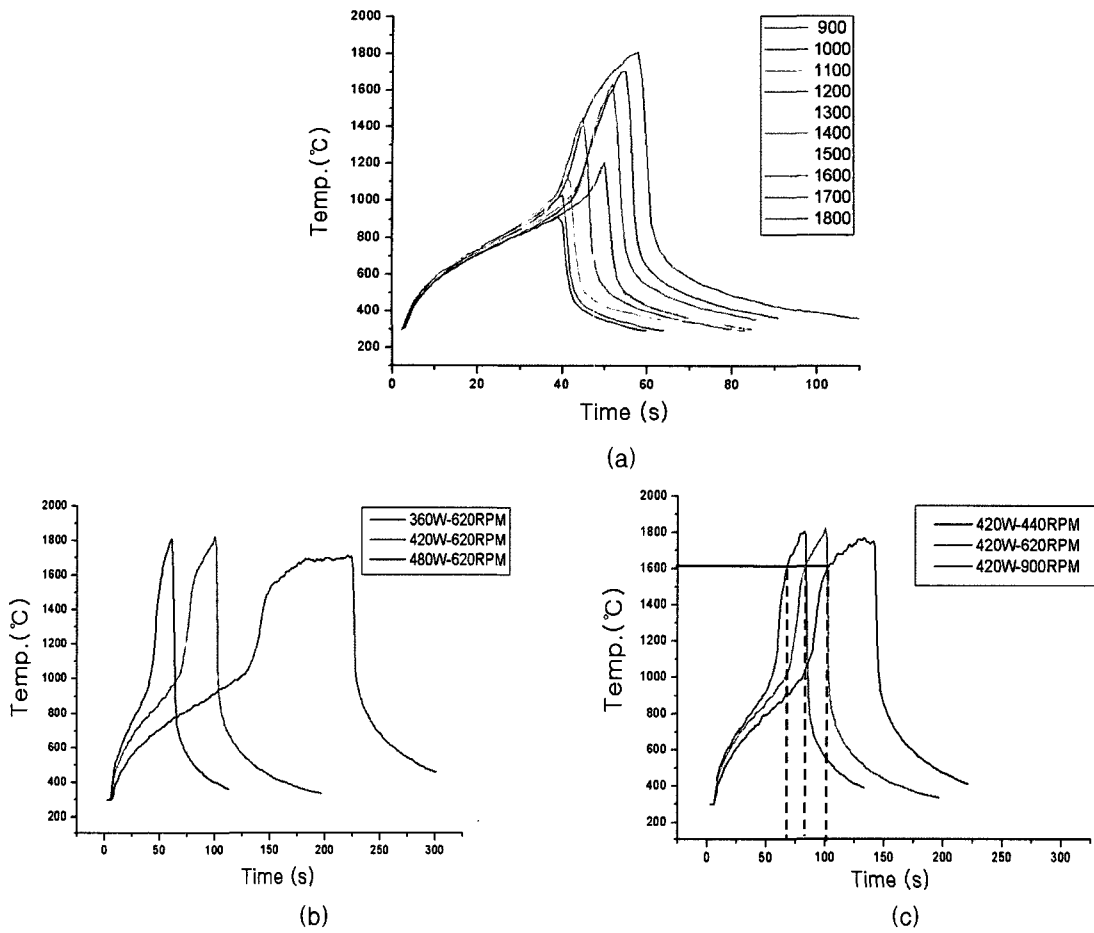
Fig. 2 Measured temperature of Si 3 N 4 according to : (a) No.9 condition from 900°C to 1800°C (b) Various power conditions at 620RPM (c) Various RPM conditions at 420W
