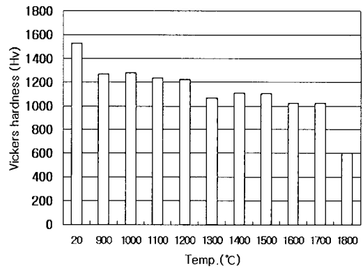
Fig. 6 The Vickers hardness of irradiated Si 3 N 4 under the No.5 condition
