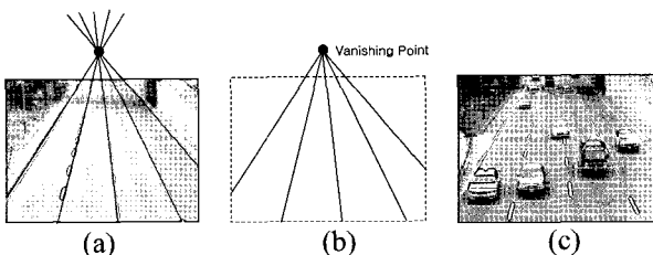
Fig. 9. Finding Vanishing Point (a) Intersecting road lanes; (b) vanishing point; (c) 3-D fitting by vanishing point
