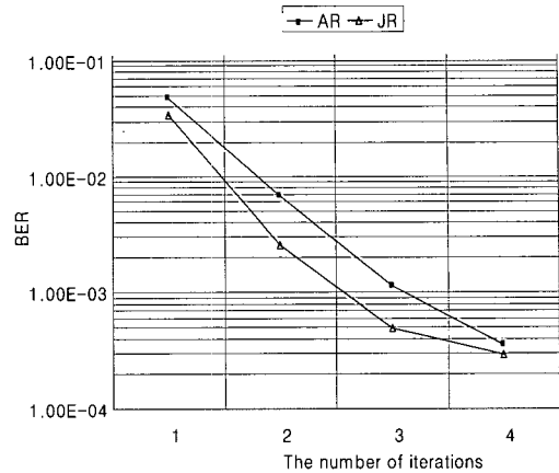
Fig. 4. BER performance of the proposed algorithm as a function of the number of iterations (JR decoding method or AR decoding method, E_b/N_0 :3.0dB, block size: 512)
