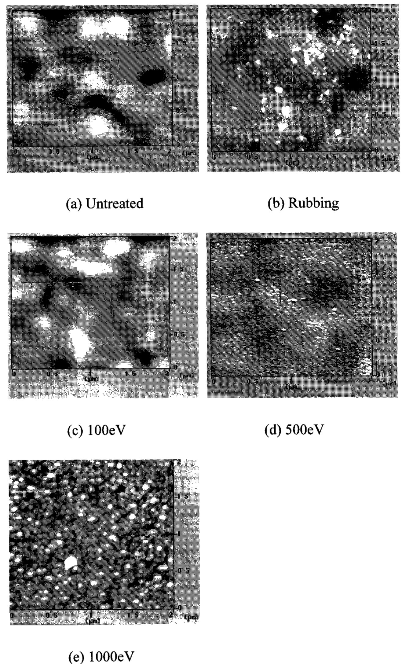
Fig. 1. Surface images by AFM
