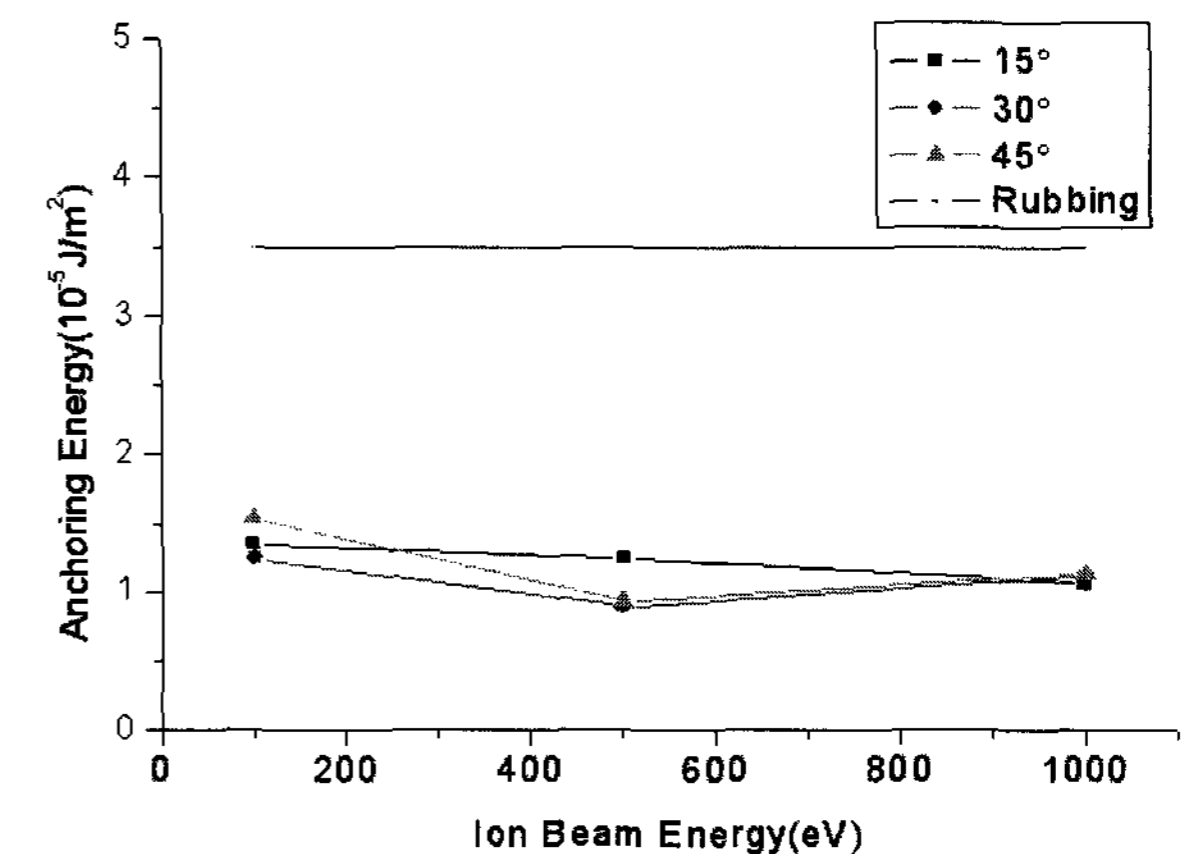
(c) Azimuthal anchoring energy for RN-1702
