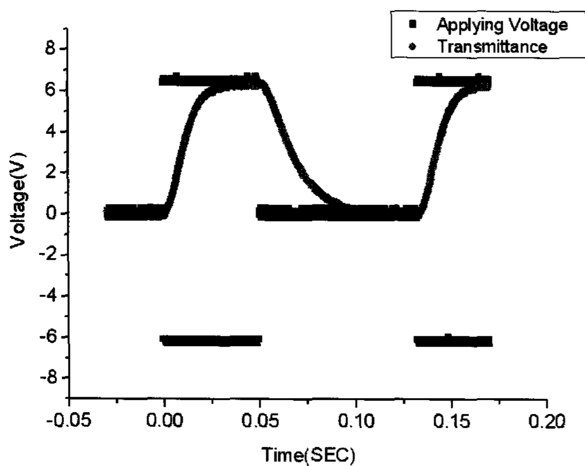
(b) rubbing-aligned IPS cell
