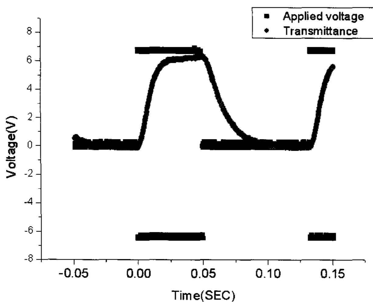
(a) Ion Beam-aligned IPS cell
