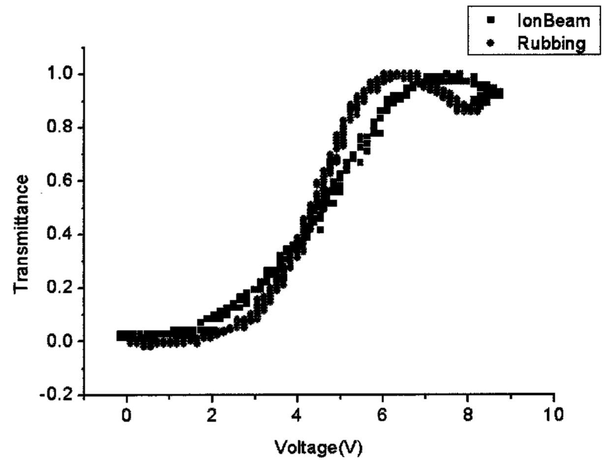
Fig. 7. Voltage-transmittance measurement.
