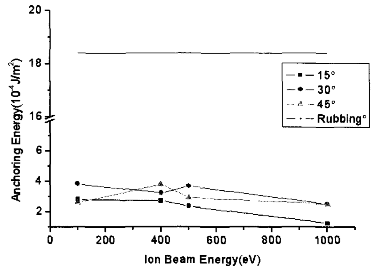
(a) Polar anchoring energy for RN-1702
