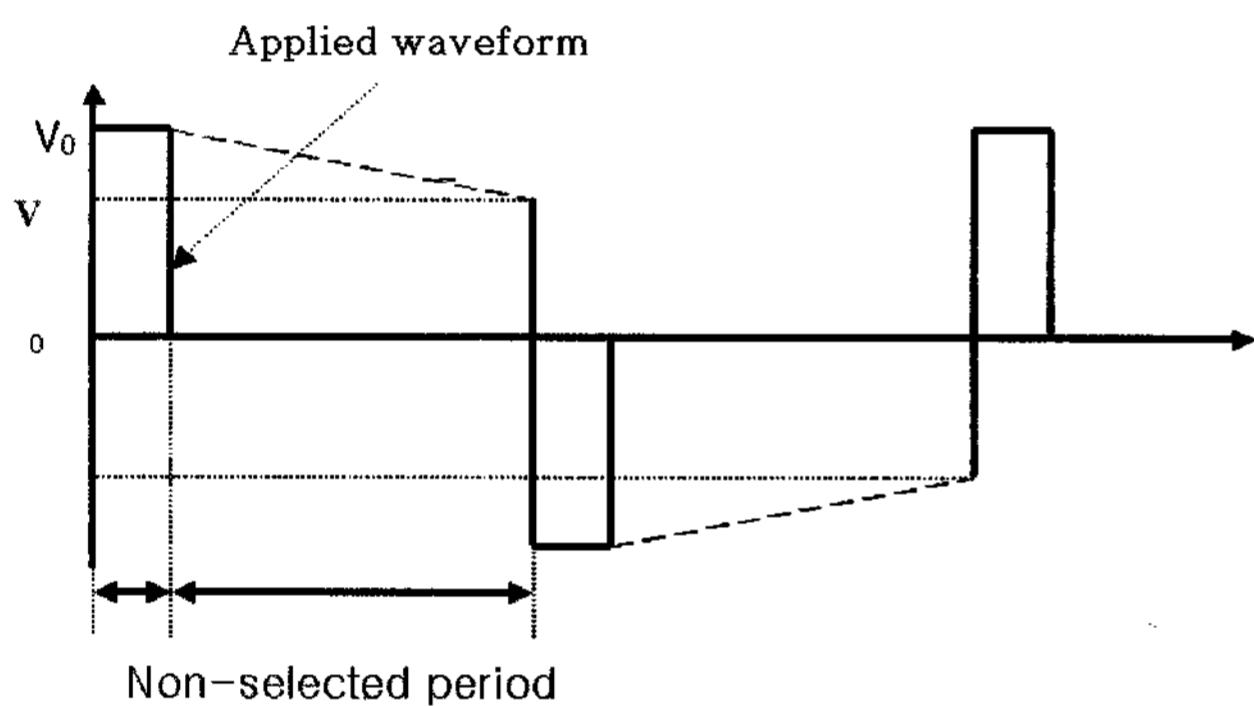
(a) Applied voltage waveform
