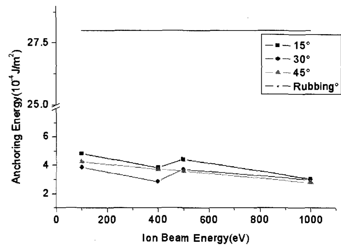
(b) Polar anchoring energy for PIA-5310
