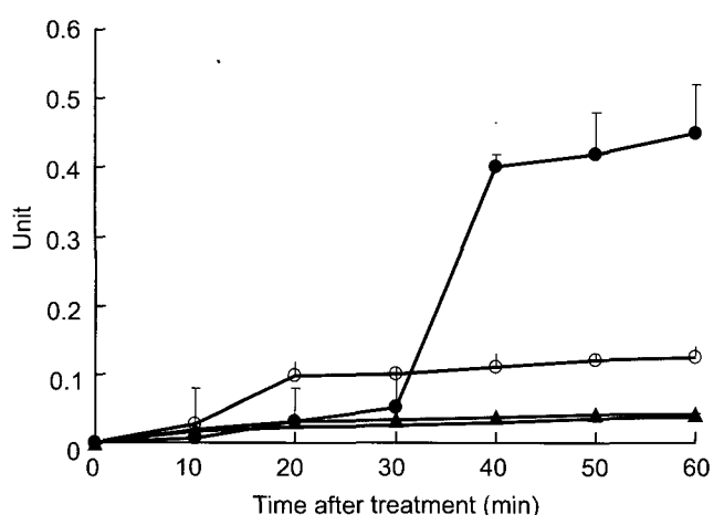
Fig. 3. \beta Gal activities in HBP01 and HBP02 strains. Samples were prepared from exponentially growing strains (open symbols). For the 1 mM hydrogen peroxide treatment (closed symbols), samples were prepared from the same phase. \beta Gal activity was measured as described in Materials and Methods. \beta Gal activity of HBP01 strain without and with treatment of hydrogen peroxide is indicated by \Delta and \blacktriangle . In the HBP02 strain, this is indicated by \circ and \bullet , respectively. Units were calculated according to the formula: 1000 \times A_{420}/\text{reaction time (min)} \times \text{OD}_{595} of culture.
