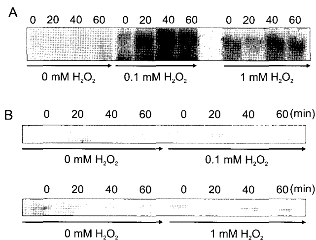
Fig. 4. The Northern blot (A) and Western blot (B) of ylaC . Exponentially growing B. subtilis PS832 was treated with 0.1 and 1 mM hydrogen peroxide. Total RNA (25 \mu g) and crude cells (20 \mu g) were prepared from B. subtilis PS832 at the indicated times and detected via Northern hybridization and Western blotting, using probes specific to ylaC and anti-YlaC antibody, respectively.
