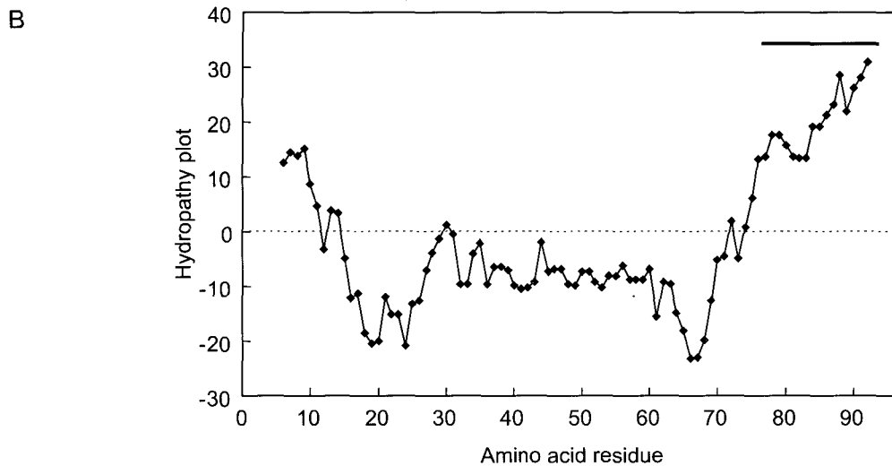
Fig. 2. Alignment of the amino acid sequences of YlaD and YlaD-related proteins and hydropathy plot for the structural prediction of YlaD. (A) The deduced amino acid sequence of YlaD (BsuYlaD) was aligned with those of M. tuberculosis OrfH (MtuOrfH), M. xanthus OrfE (MxaOrfE) and S. coelicolor RsrA (ScoRsrA). The positions of the conserved amino acids are marked by asterisks and colons for identical and similar matches, respectively. (B) The hydropathy of each of the amino acid residues was calculated via the methods developed by Kyte and Doolittle, using a window size of 11 residues. The solid bar in the plot indicates the segment predicted to form transmembrane helices.
