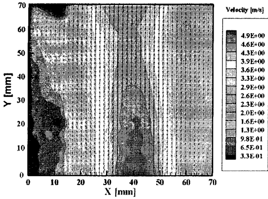
Fig. 5 Mean velocity fields in the 3rd region of Case 1 at the fluid speed 7 m/s in the muffler inlet (z surface : ③)
