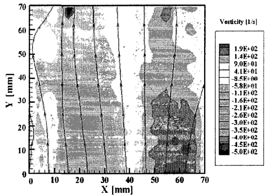
Fig. 11 Mean vorticity fields in the 3rd region of Case 1 at the fluid speed 7 m/s in the muffler inlet (z surface : ③)
