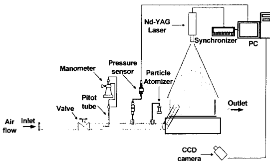
Fig. 1 Schematic diagram for PIV measurement
