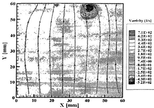
Fig. 14 Mean vorticity fields in the 3rd region of Case 2 at the fluid speed 7 m/s in the muffler inlet (z surface : ③)
