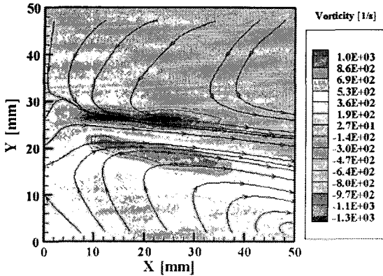
Fig. 13 Mean vorticity fields in the 6th region of Case 1 At the fluid speed 3.5 m/s in the muffler inlet (z surface : ⑥)
