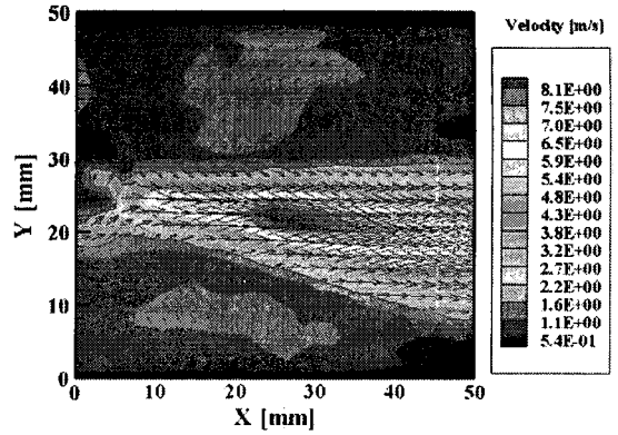
Fig. 7 Mean velocity fields in the 6th region of Case 1 at the fluid speed 3.5 m/s in the muffler inlet (z surface : ⑥)
