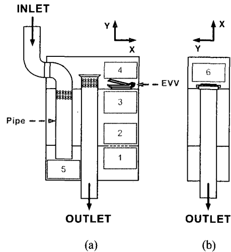
Fig. 4 The measurement region in the visualization muffler
