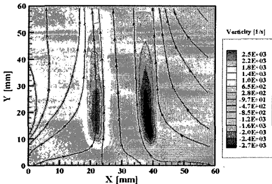
Fig. 15 Mean vorticity fields in the 4th region of Case 2 at the fluid speed 7 m/s in the muffler inlet (z surface : ④)
