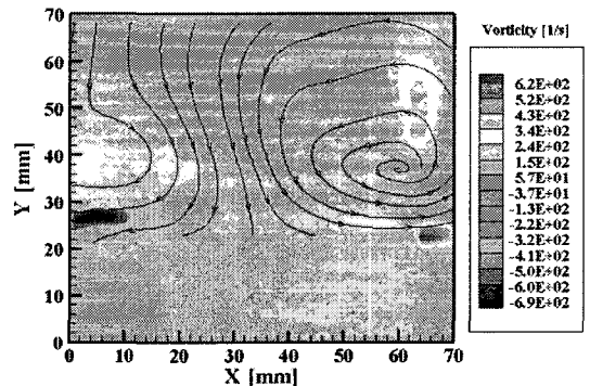
Fig. 12 Mean vorticity fields in the 4th region of Case 1 at the fluid speed 7 m/s in the muffler inlet (z surface : ④)
