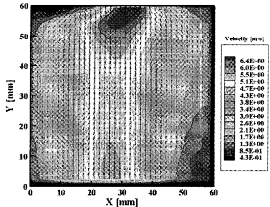
Fig. 8 Mean velocity fields in the 3rd region of Case 2 at the fluid speed 7 m/s in the muffler inlet (z surface : ③)
