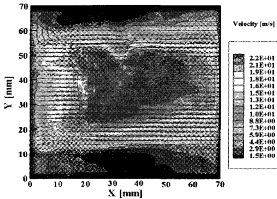
Fig. 10 Mean velocity fields in the 6th region of Case 2 at the fluid speed 7 m/s in the muffler inlet (z surface : ⑥)
