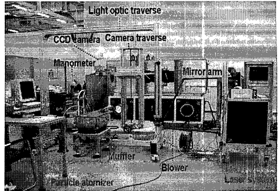
Fig. 2 View of PIV experimental equipment
