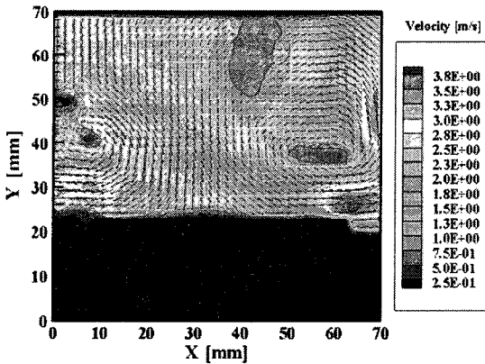
Fig. 6 Mean velocity fields in the 4th region of Case 1 the fluid speed 7 m/s in the muffler inlet (z surface : ④)
