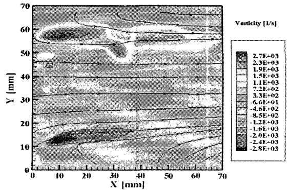
Fig. 16 Mean vorticity fields in the 6th region of Case 2 at the fluid speed 7 m/s in the muffler inlet (z surface : ⑥)
