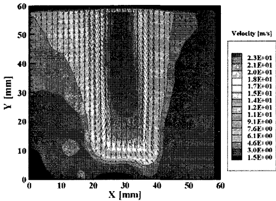
Fig. 9 Mean velocity fields in the 4th region of Case 2 at the fluid speed 7 m/s in the muffler inlet (z surface : ④)
