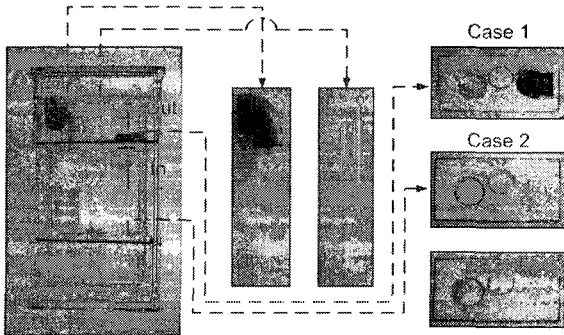
Fig. 3 Experimental apparatus of the visualization muffler
