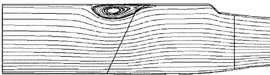
Fig. 9 Streamline distributions for the backward-sweep inducer at 120%Q d
