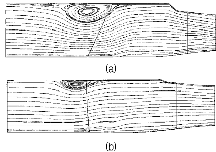
Fig. 5 Streamline distributions at 100\%Q_d : (a) backward-sweep inducer (b) forward-sweep inducer
