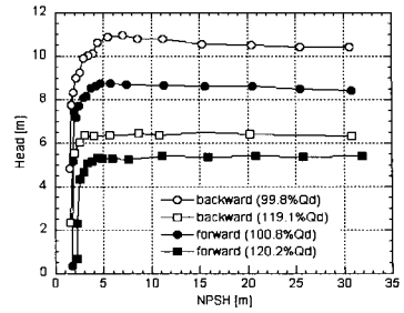
Fig. 8 Suction performances
