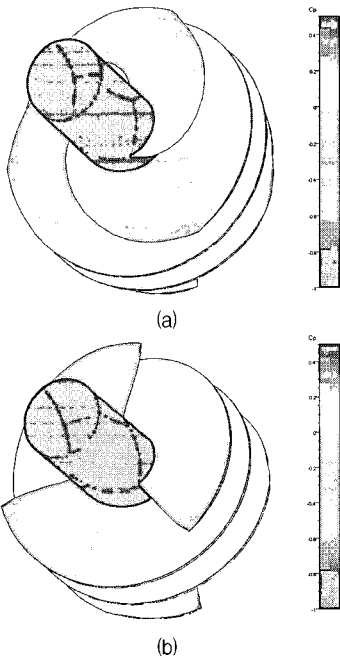
Fig. 4 Static pressure coefficient distributions : (a) backward sweep inducer (b) forward sweep inducer
