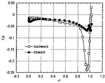
Fig. 6 Inlet pressure coefficient distributions
