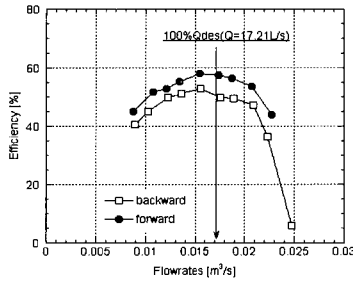
Fig. 7 Efficiency distributions
