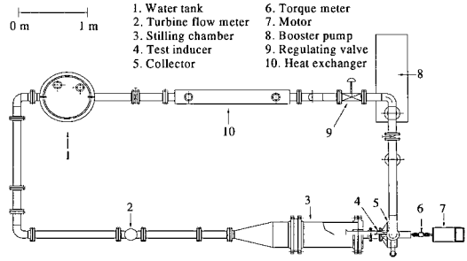
Fig. 2 Plane view of the test loop
