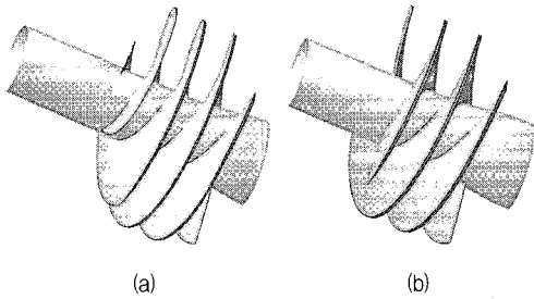
Fig. 3 Backward and forward inducers : (a) backward (b) forward
