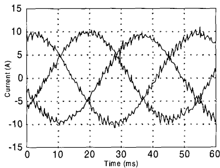
(c) Current
