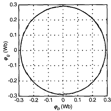
(b) Flux
