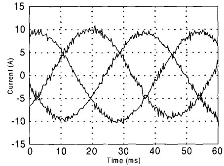
(c) Current
