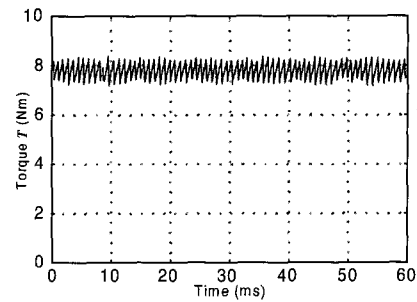
(a) Torque
