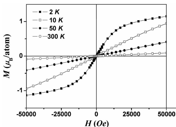
Figure 5. The M - H curves at T = 2, 10, 50, and 300 K.
