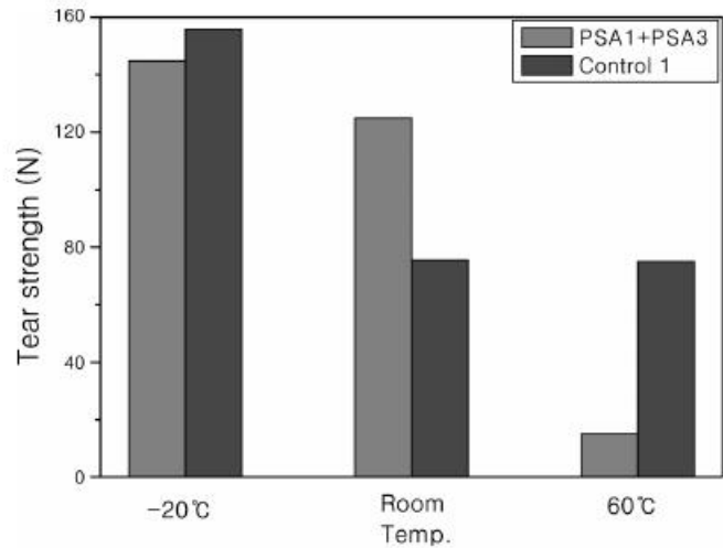
Figure 10. Tear force of PSA-bonded assembly parts used in automobile industry.
