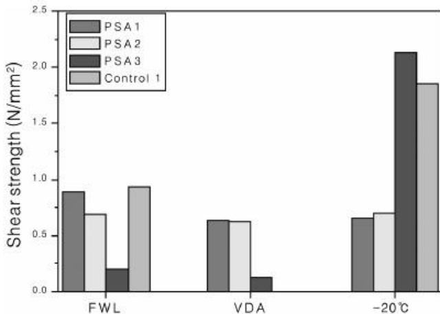
Figure 9. Effect of aging conditions on single lap shear strength.
