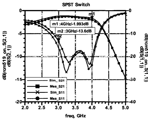
(b) 스위치 Off-State 측정 결과 (b) Measured result of the switch under Off-state
