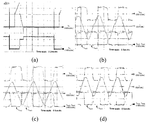
Fig. 15 Voltage and current waveforms of the proposed high frequency driver: (a) Voltage waveforms across panel during 1 subfield (b) sustaining waveform with 500kHz switching freq (c) sustaining waveform with 600kHz switching freq (d) sustaining waveform with 700kHz switching freq
