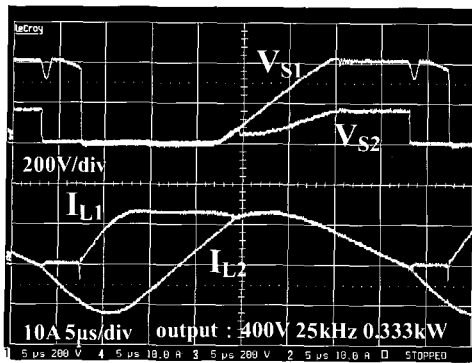
Fig. 9 The test result of the current discontinuous mode
