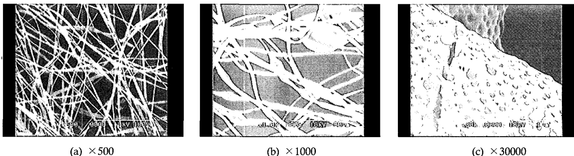
Figure 1. SEM micrographs of MWNT/PMMA(0.5 wt%/10 wt%) nanofibers electrospun from chloroform. (a)×500, (b)×1000, and (c)×30000.
