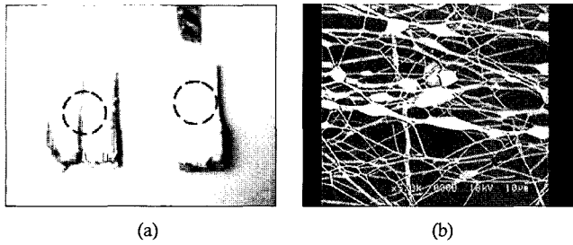
Figure 6. (a) Separated electrodes and electrospun fibers and (b) SEM micrographs of MWNT/PMMA (0.5 wt%/10 wt%) aligned nanofibers electrospun from DMF ( \times 5000 ).
