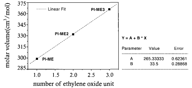
Figure 14. Linear dependency of molar volume on the number of carbon
