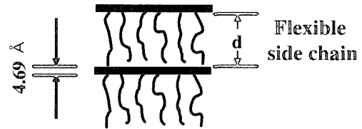
Figure 15. Proposed structure of PI-ME series(Layered structure of single backbone).
