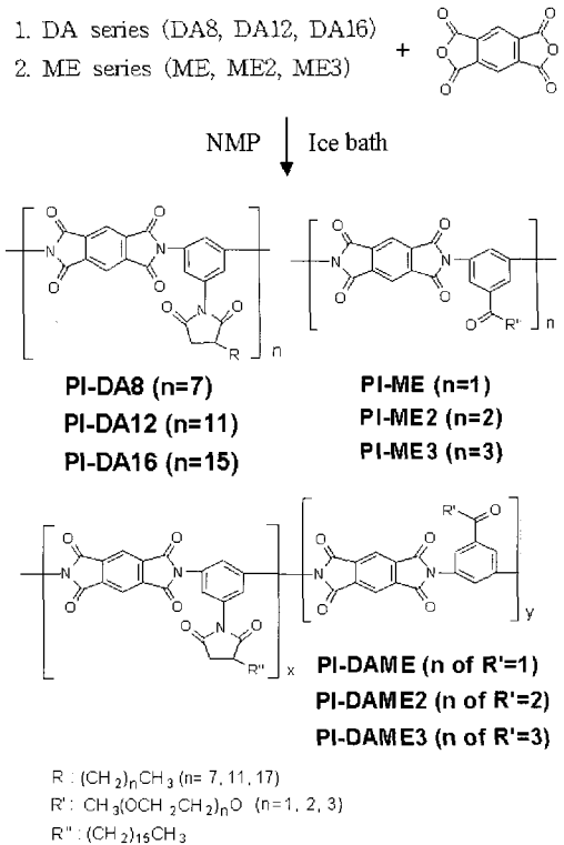
Scheme 2. Synthesis of polyimides containing flexible side chain.
