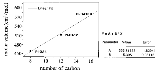
Figure 7. Linear dependency of molar volume on the number of carbon.
