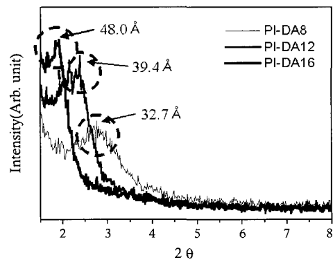
Figure 3. X-ray diffractograms of PI-DA series.
