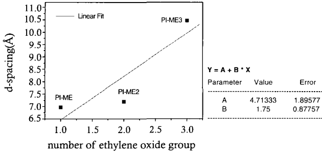
Figure 13. Linear dependency of d-spacing on the number of ethylene oxide unit.
