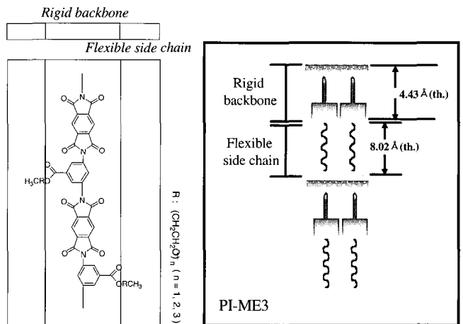
Figure 11. Calculation of chain length of layered structure.
