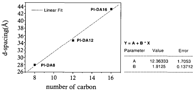
Figure 6. Linear dependency of d-spacing on the number of carbon.
