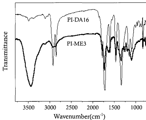
Figure 2. IR spectra of PI-DA16 & PI-ME3.
