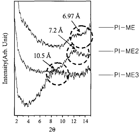
Figure 9. X-ray diffractograms of hydrophilic series.
