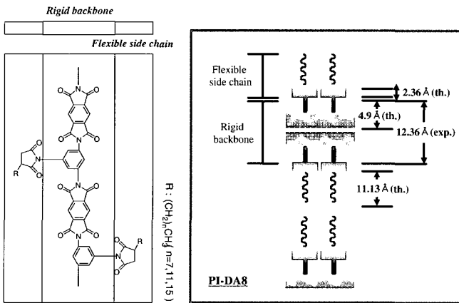
Figure 4. Calculation of chain length of layered structure.
