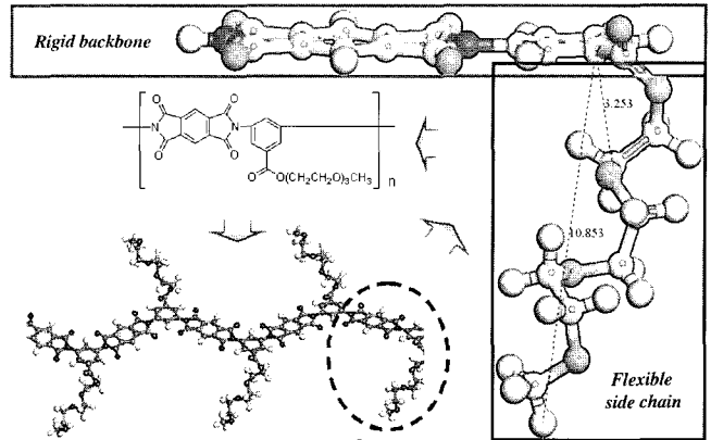
Figure 10. Molecular modeling through Material Studio.
