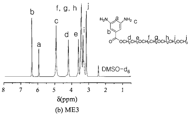
Figure 1. 1 H-NMR spectra of diamine.
