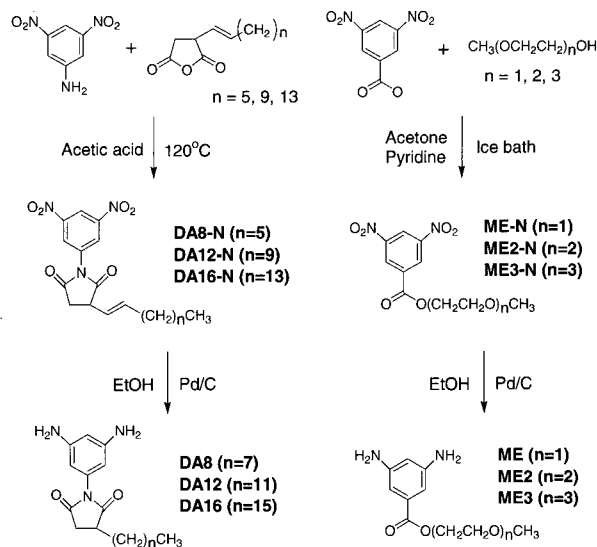
Scheme 1. Synthesis of the monomers.
