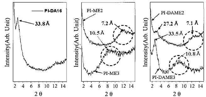
Figure 16. X-ray diffractograms of segregated layered structure.
