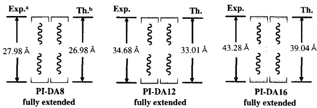
Figure 5. Models of flexible side chain in layered structure a Experimental calculation; b Theoretical calculation).
