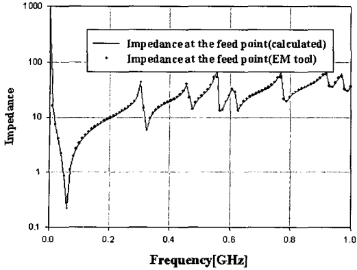
Fig. 2. Input impedance profile of the DC power bus without loading(calculated and compared to other method).
