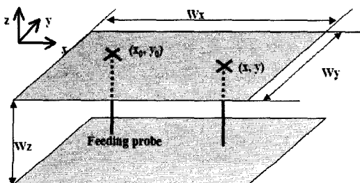
Fig. 1. DC power bus modelled as a cavity.
