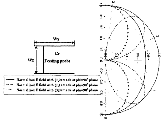
(a) Radiated field at \phi=0^\circ plane
