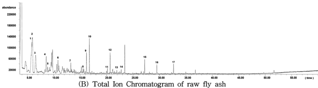
Fig. 3. GC/MSD extraction ion chromatograms of residues from Municipal Solid Wastes Incinerator.
