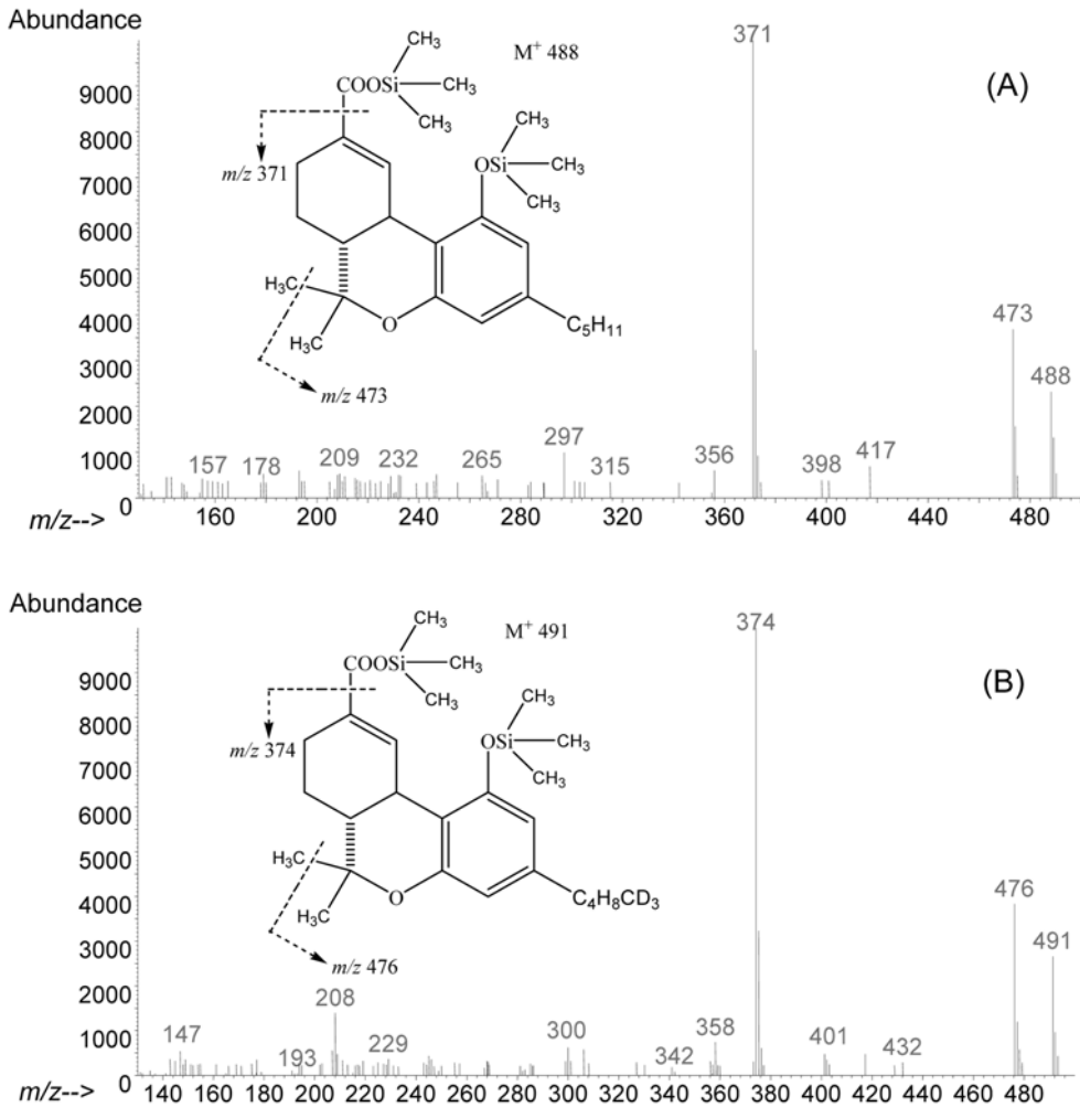
Fig. 3. EI mass spectra of TMS derivatives of (A) THCCOOH and (B) THCCOOH-d 3 .
