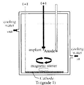
Fig. 2. Schematic drawing of anodizing apparatus.
