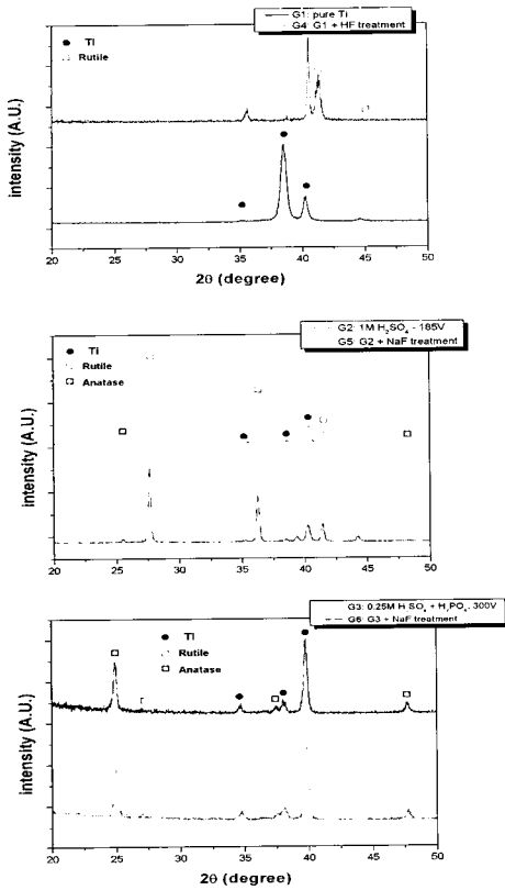
Fig. 12. X-ray diffractometer patterns of six treated groups.
