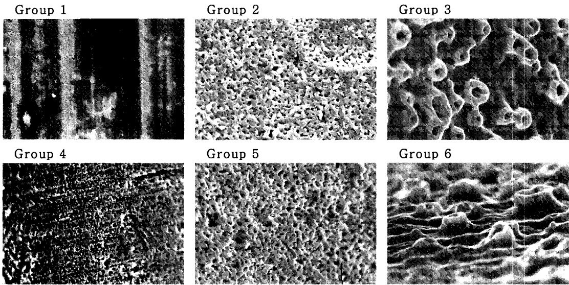
Fig. 8. SEM images of each specimen (magnification of X3,000).
