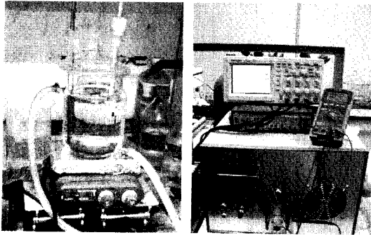
Fig. 3. Anodizing apparatus used in this specimens experiment.
