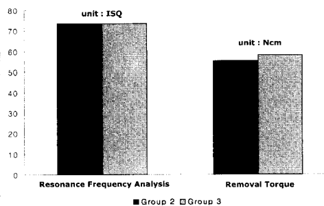
Fig. 24. Implant stability according to anodic oxidized processing methods.
