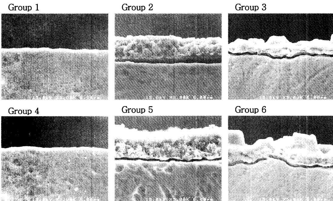
Fig. 9. Cross-sectional SEM images of each specimen (magnification of X5,000).
