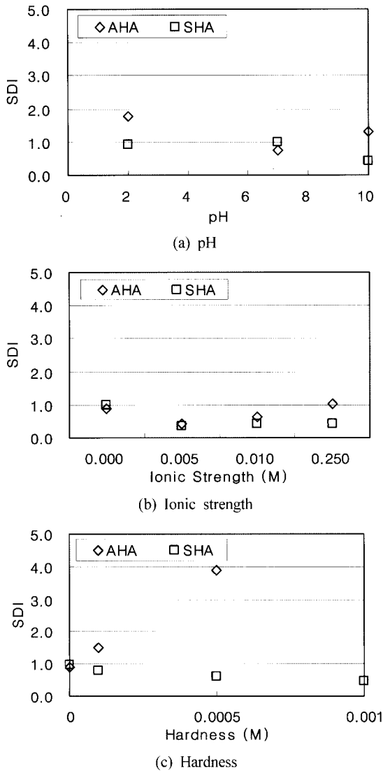
Fig. 6. Effect of solution chemistry on SDI.
