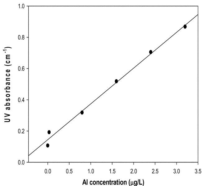
Fig. 2. Correlation of absorbance and standard Al solutions.
