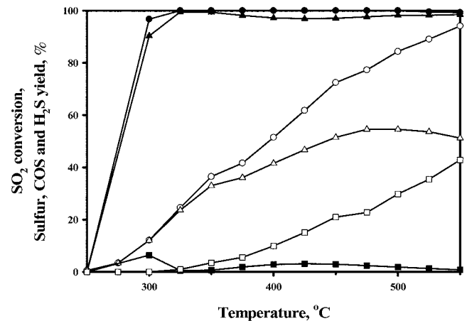
Fig. 6. Effect of temperature on the SO 2 reduction by CO or H 2 over SnO 2 -ZrO 2 (Sn/Zr=3/1)(●: SO 2 conversion-CO, ○: SO 2 conversion-H 2 , ▲: Sulfur yield-CO, △: Sulfur yield-H 2 , ■: COS yield-CO, □: H 2 S yield-H 2 ).
