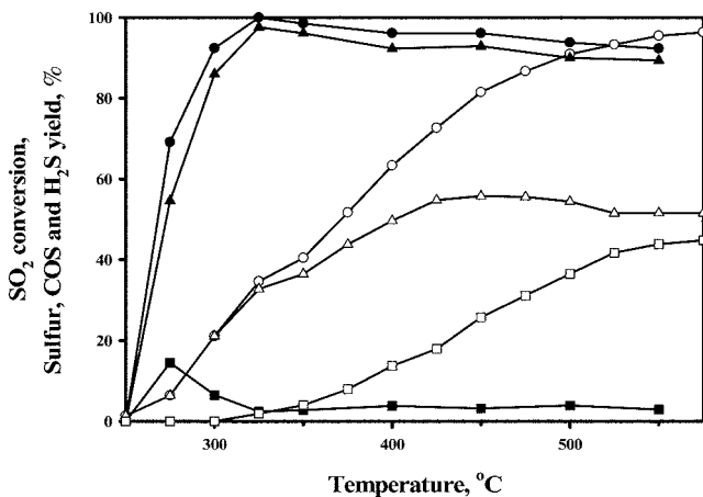
Fig. 5. Effect of temperature on the SO 2 reduction by CO or H 2 over SnO 2 -ZrO 2 (Sn/Zr=2/1)(●: SO 2 conversion-CO, ○: SO 2 conversion-H 2 , ▲: Sulfur yield-CO, △: Sulfur yield-H 2 , ■: COS yield-CO, □: H 2 S yield-H 2 ).
