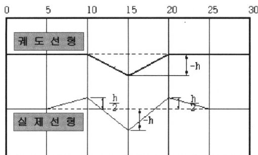
그림 1. Comparison between real geometry and recording data
