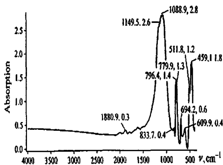
Fig.2. IR spectroscopy of quartz activated within 10 min.
