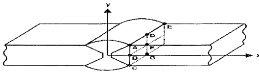
Fig. 6 Butt weld specimen
