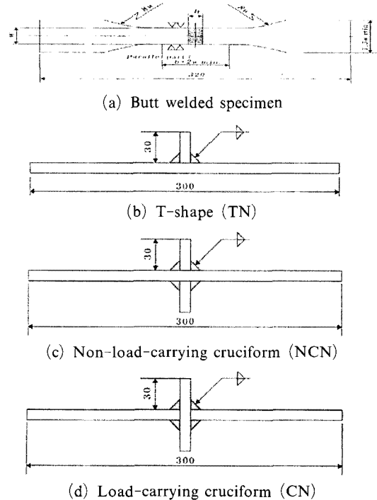
Fig. 1 Specimens for test and analysis
