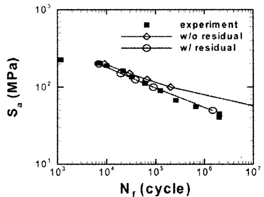
Fig. 12 Load-carrying cruciform (CN)
