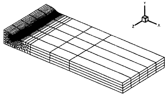
(a) Butt welded specimen
