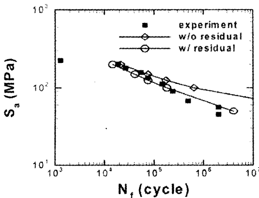
Fig. 11 Non-load-carrying cruciform (NCN)
