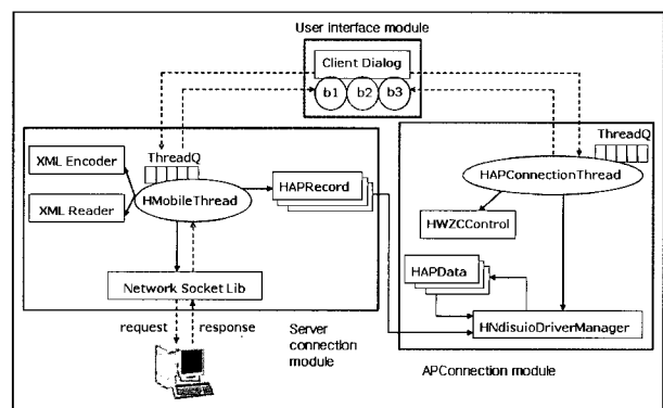
Fig. 3. Client software
