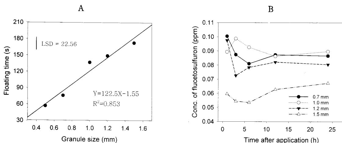
Fig. 3. Floatation of the floating granules (A) and dispersal of flucetosulfuron (B) as affected by granule size. The concentration of flucetosulfuron was measured at 7 m apart from the application point. Template formulation: flucetosulfuron, Surfynol 440, SPA, xanthan gum, and potassium chloride to 100%.
