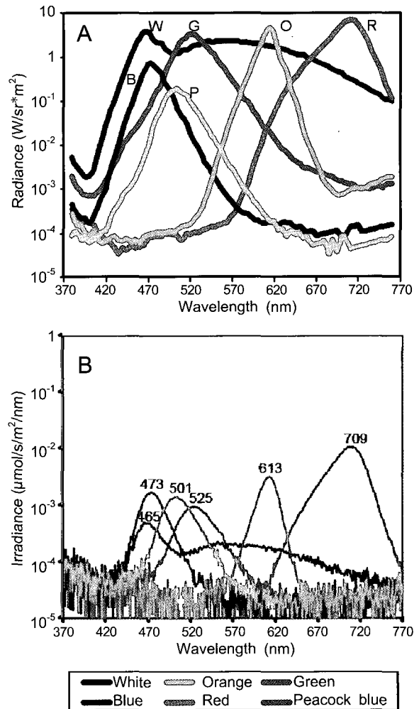
Fig. 6. Change of spectral radiance (A) and spectral irradiance (B) according to the high-luminance light-emitting diode light source.
