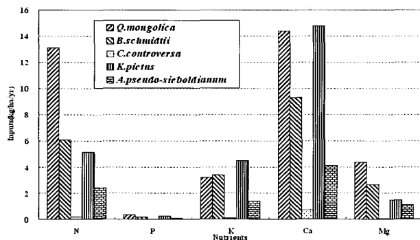
Fig. 4. Nutrient inputs ( \text{kg ha}^{-1} \text{ yr}^{-1} , n=3 ) by leaf litter of main species for 3 years at the LTER site in Mt. Gyeongbansan.
