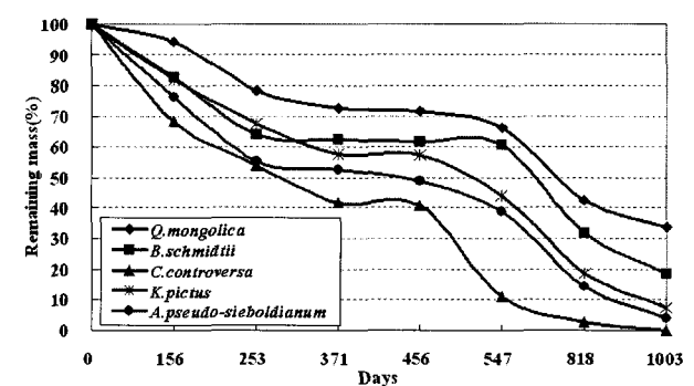
Fig. 5. Remaining mass (% , n=4 ) of leaf litter for three years at the LTER site in Mt. Gyeongbansan.
