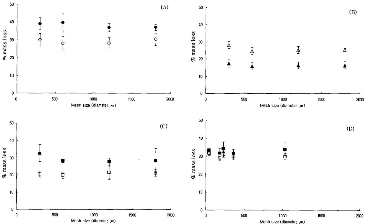
Fig. 5. Changes in mass loss (Mean±SD, n=4) of each part of emergent macrophytes species according to the different mesh size at first experiment (A, Z. latifolia ; B, P. communis ; C, T. angustata ) for 42days from Sep. 22 to Nov. 2, 2005, and second experiment (D, T. angustata ) for 40 days from Apr. 3 to May 12, 2006 at 1m depth of water of vegetated floating island in Lake Paldang. Culms are black and blades are white. Differences have been tested by ANOVA (n=4).
