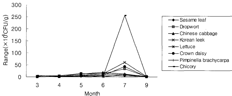
Fig. 1. Monthly variations of total aerobic bacterial counts in individual fresh vegetables.
