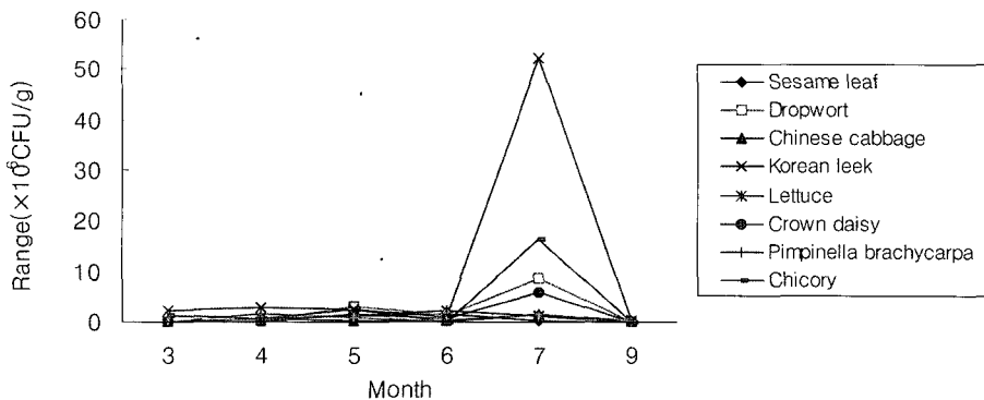
Fig. 2. Monthly variations of coliform bacterial counts in individual fresh vegetables.
