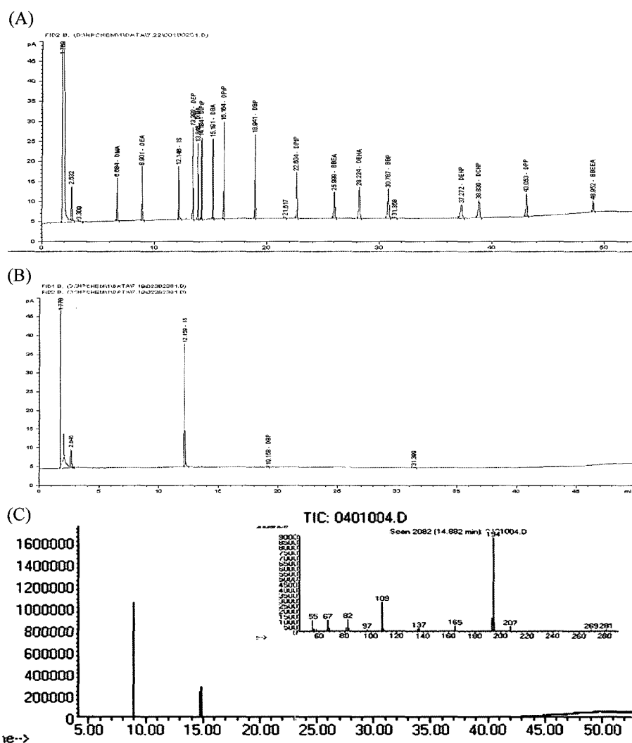
Fig. 1. Chromatogram of 16 plasticizers analyzed in tea bag filter. (A) GC/FID Chromatogram of Standard (mixture of 16 plasticizers); (B) GC/FID Chromatogram of Sample; (C) GC/MSD Chromatogram (scan mode) of Sample.
