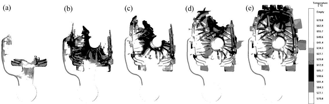
Fig. 3. Sequences of mold filling simulation (case 1).
