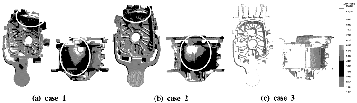
Fig. 7. Porosity defects predicted by air pressure criterion.
