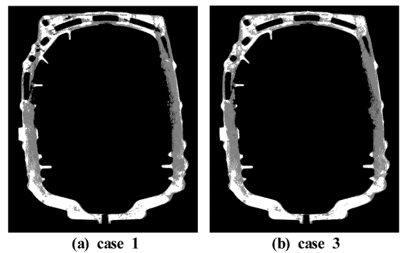
Fig. 8. Porosity defects by Computer Tomography.
