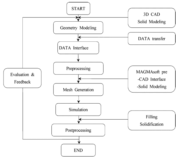
Fig. 1. Flow-chart of die casting simulation.
