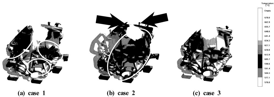
Fig. 6. Final flow junction zone.
