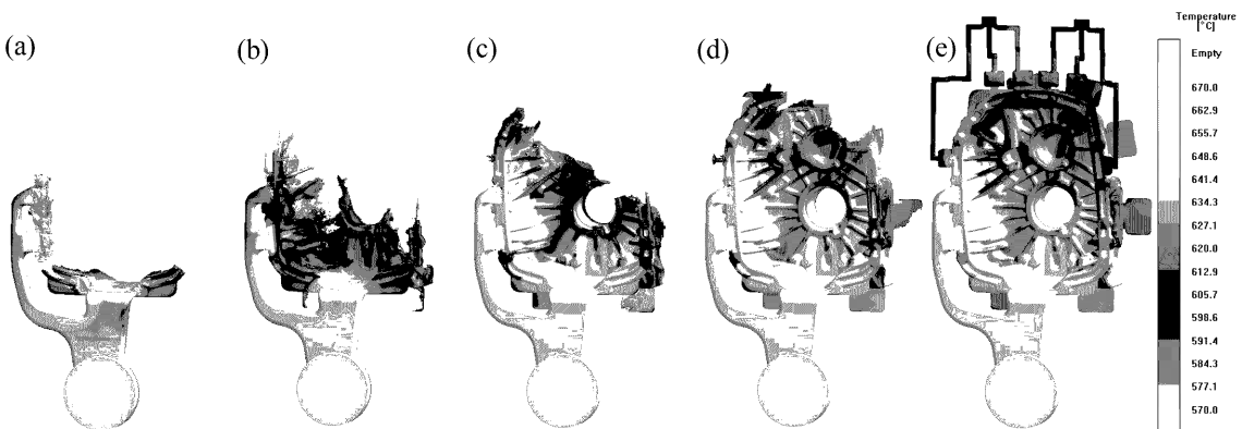
Fig. 5. Sequences of mold filling simulation (case 3).
