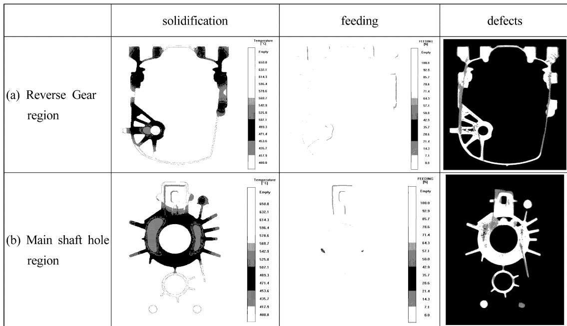
Fig. 11. Shrinkage defects predicted by solidification and feeding criterion.
