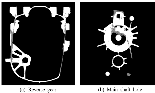
Fig. 14. CT photographing results by Local squeeze effect.
