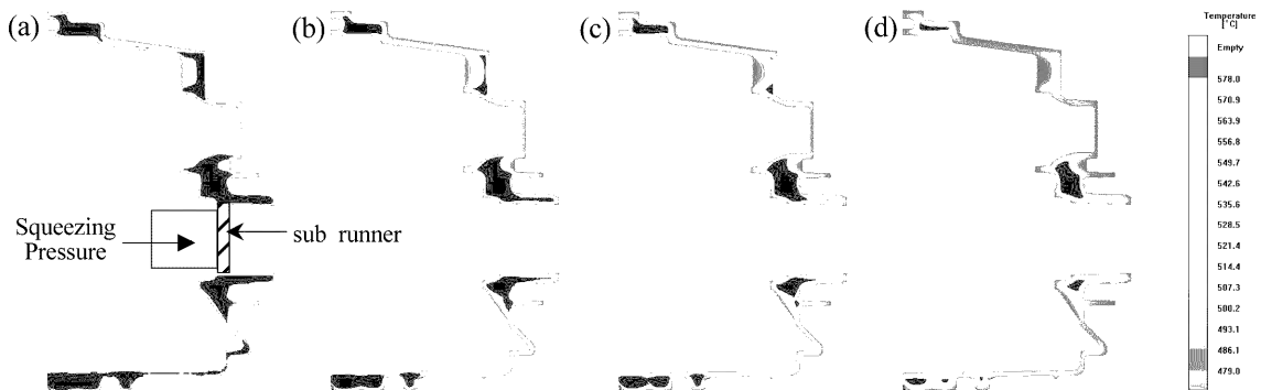
Fig. 12. Solidification simulation of main shaft hole region for the squeeze time design.
