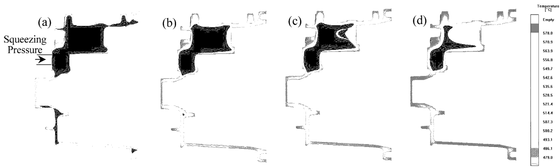
Fig. 13. Solidification simulation of reverse gear region for the squeeze time design.
