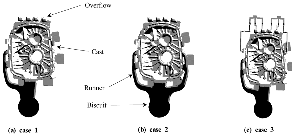
Fig. 2. Casting design of gear housing.
