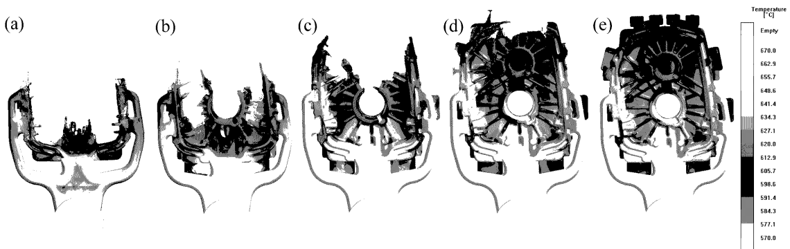
Fig. 4. Sequences of mold filling simulation (case 2).
