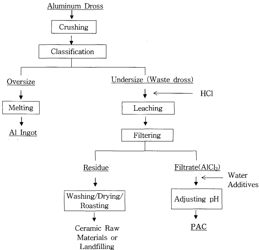
Fig. 1. Schematic process flow sheet for preparing PAC from aluminum dross.
