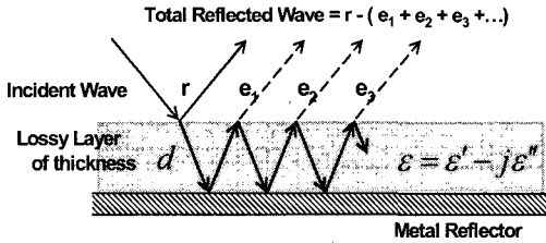
Fig. 4 Schematic drawing of the single-layer absorber.
