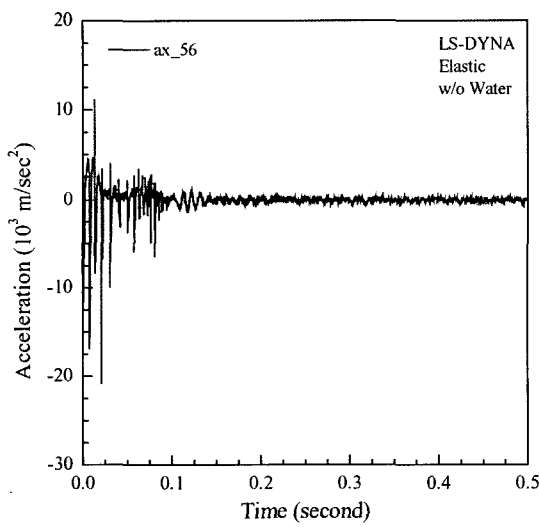
Fig. 10. Response Time Histories of Impact Point for LS-DYNA Elastic Analysis without Water
