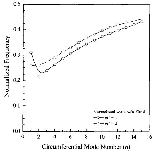
Fig. 4. Normalized Frequencies of Tank with Fluid with Respect to Without-Fluid
