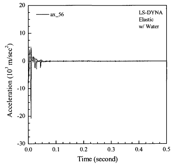
Fig. 11. Response Time Histories of Impact Point for LS-DYNA Elastic Analysis with Water (by Coupling Fluid with Shell using CPINTF)
